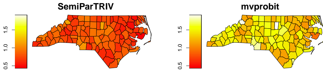
Fig. 2: Joint probabilities (in %) that mb is multiple, lbw is > 2500 grams and ptb is > 37 weeks by county in North Carolina, obtained using by SemiParTRIV() and mvprobit() .
