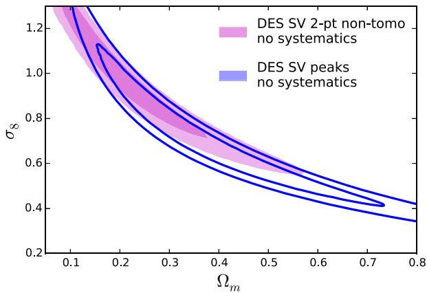
Figure 6. Comparison between constraints from peak statistics (blue solid lines) and shear 2-pt functions (pink contours), with systematics excluded. Both constraints show the 68 and 95 per cent confidence limits. To make a fair comparison, we did not marginalize other parameters for the 2-pt constraints and we set h = 0.7 , \Omega_b = 0.04 and n_s = 1 , to match the configuration for simulations.
