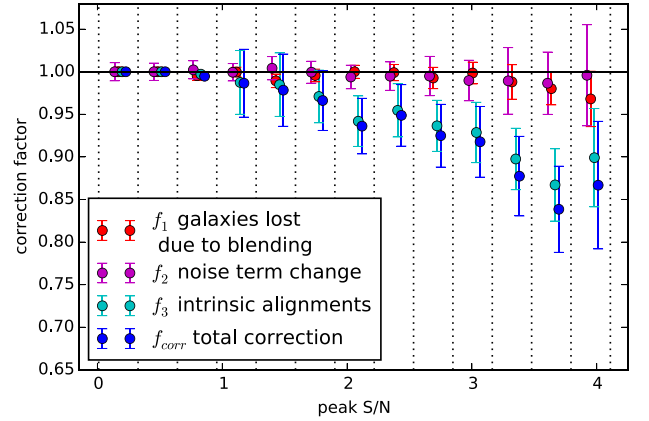
Figure C3. Boost factor and IA corrections for all S/N bins used in the analysis. Error bars on these factors are propagated from the errors on f_{\text{cluster}} and f_{\text{lost}} .
