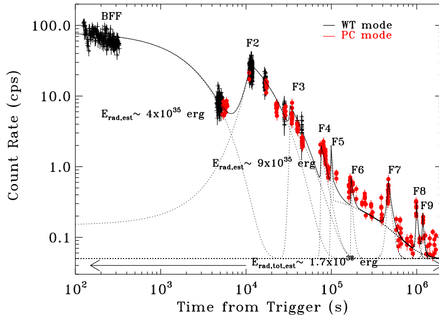
Figure 5. Swift XRT light curve of the coverage of the initial trigger and subsequent flaring activity of DG CVn over the following \sim 21 days. Because of gaps in the data, exponential rises and decays were used to approximate the observed behavior, and the models were integrated in time to estimate flare radiated energies in the 0.3–10 keV bandpass.
