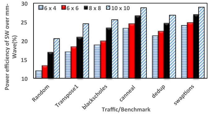
Fig. 14. Average network power efficiency.
