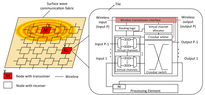
Fig. 2. Hybrid wireline-surface wave NoC architecture.
