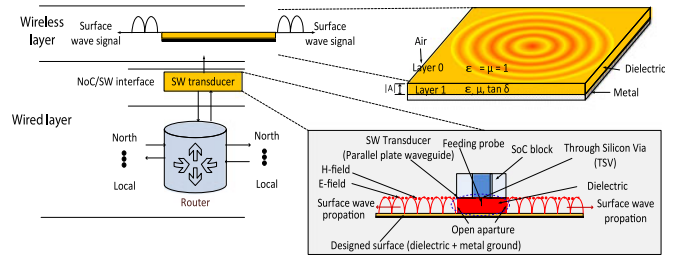
Fig. 4. Interface between the 2-D guided wave channel and the wireline channel.
