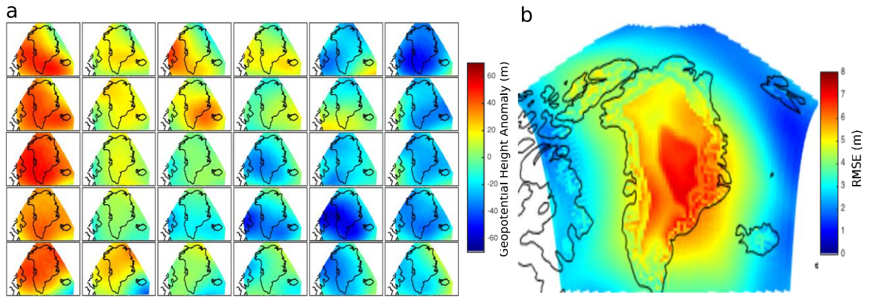
Fig. 3: (a) MAR 500 hPa height anomalies mapped to their best matching node and averaged over all dates. (b) Root Mean Square Error of node-averaged MAR 500 hPa geopotential height anomalies from those of MERRA after regridding.
