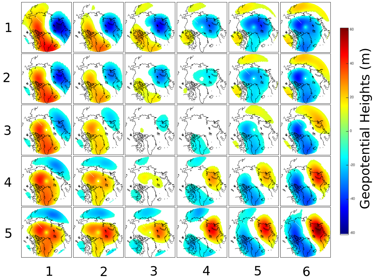
Fig. 1: Master map of SOM nodes obtained from daily JJA 500 hPa geopotential height anomalies (1979-2014).
