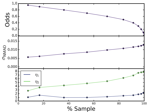
Figure 11. Effect of the selection of sub-samples based on the Odds parameter. Top panel: evolution of the Odds parameter with sample size. Middle panel: evolution of the photometric redshift accuracy \sigma_{\text{NMAD}} with sample size, thresholded by Odds values. Bottom panel: outlier rate parameters \eta_1 and \eta_2 as a function of sample size.
