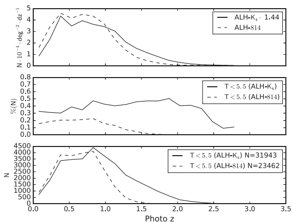
Figure 16. Top: photometric redshift distribution for the K_s -selected (solid line) and F814W -selected (dashed line) samples. Centre: fraction of galaxies in both samples whose best-fitting templates are 1 < T_B < 5.5 , which we identify as early-type SEDs. Bottom: absolute number of early-type sources at each redshift in each catalogue.
