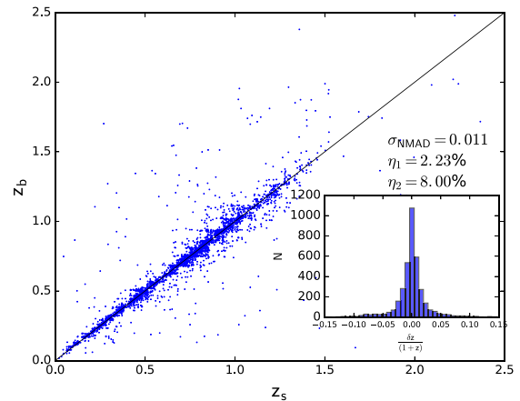
Figure 10. ALHAMBRA K_s photometric redshift z_b versus spectroscopic redshift z_s for 3736 sources. The inset shows the distribution of the deviations \delta z / (1+z) . The measured scatter is \sigma_{\text{NMAD}} = 0.011 , with catastrophic error rates \eta_1 \sim 2.3 per cent, \eta_2 \sim 8.0 per cent.
