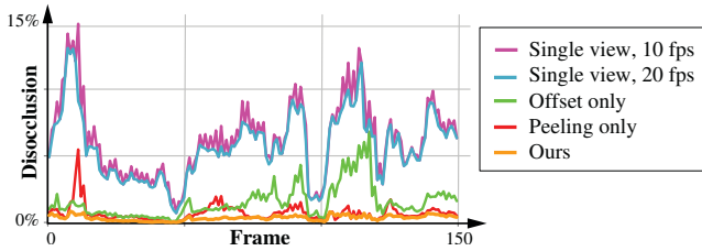
Figure 4: Fraction of missing pixels during a walkthrough of the VIKING VILLAGE as seen in Figure 5.
