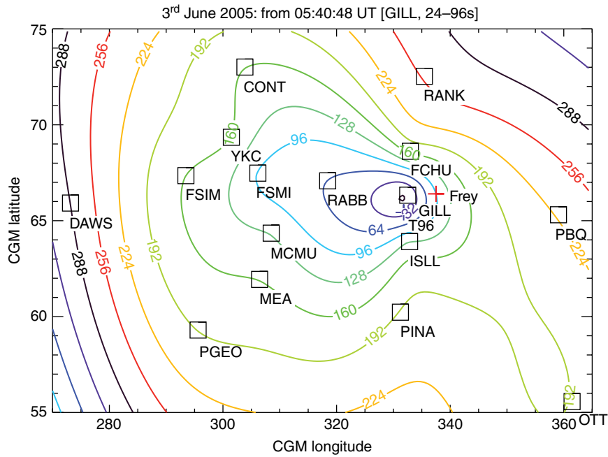
Figure 7.4 Arrival time of Pi1-2 ULF waves as in Figure 7.3 from Murphy et al. [2009] , but as compared to the location of auroral brightening observed by the IMAGE FUV instrument from the Frey substorm list [ Frey and Mende, 2007 ].
