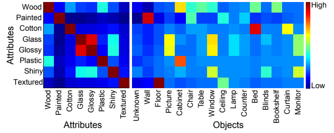
Fig. 3. Visualization of the R^{\mathcal{O},\mathcal{A}}, R^{\mathcal{A},\mathcal{A}} terms used to encode object-attribute and attribute-attribute relationships.
