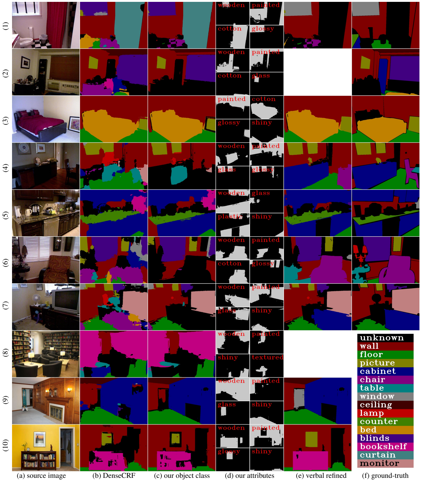
Fig. 7. Qualitative comparisons. Note that after verbal refinement, our algorithm provides results that correspond closely to human scene understanding. This is also reflected in the numerical results tabulated in Table IV. The last three images are from the Internet and lack ground truth. For the second and eighth image, there are no attribute combinations which would improve the result, hence there is no verbal refinement. (See Table II for the used verbal commands.)
