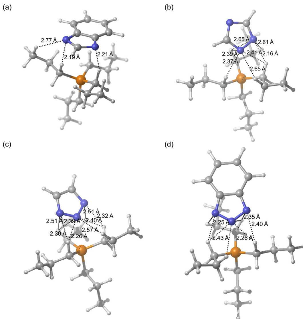
Figure 1. Ionic pairs comprising a tetrapropylphosphonium cation, [P 3333 ] + , with the four anions: (a) [P 3333 ][Benzim], (b) [P 3333 ][124Triz], (c) [P 3333 ][123Triz] and (d) [P 3333 ][Bentriz]. Dashed lines indicate intermolecular N-H distances less than or close to the sum of the vdW radii (2.75 Å) Colour code: blue – nitrogen; yellow – phosphorus; grey – carbon; white – hydrogen.
