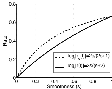
Figure 1: Comparison of the r_o(l) = l^{-\frac{2s}{2s+1}} and r(l) = l^{-\frac{2s}{s+2}} rates as function of the problem difficulty/smoothness ( s ).
