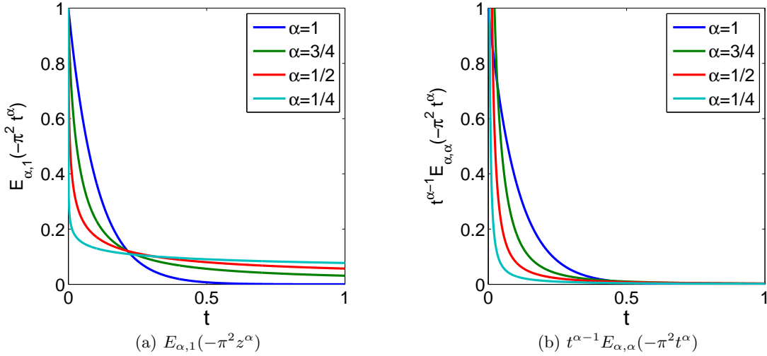
FIGURE 1. The profiles of Mittag-Leffler functions (a) E_{\alpha,1}(-\pi^2 z^\alpha) and (b) t^{\alpha-1}E_{\alpha,\alpha}(-\pi^2 t^\alpha) . The value \pi^2 is the first Dirichlet eigenvalue of the negative Laplacian on the interval (0, 1) .
