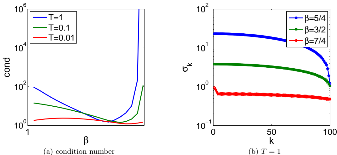
FIGURE 15. Numerical results for the space fractional sideways problem, with the lateral Cauchy data at the point x = 1 : (a) the condition number v.s. the fractional order \beta and (b) the singular value spectrum at T = 1 .
