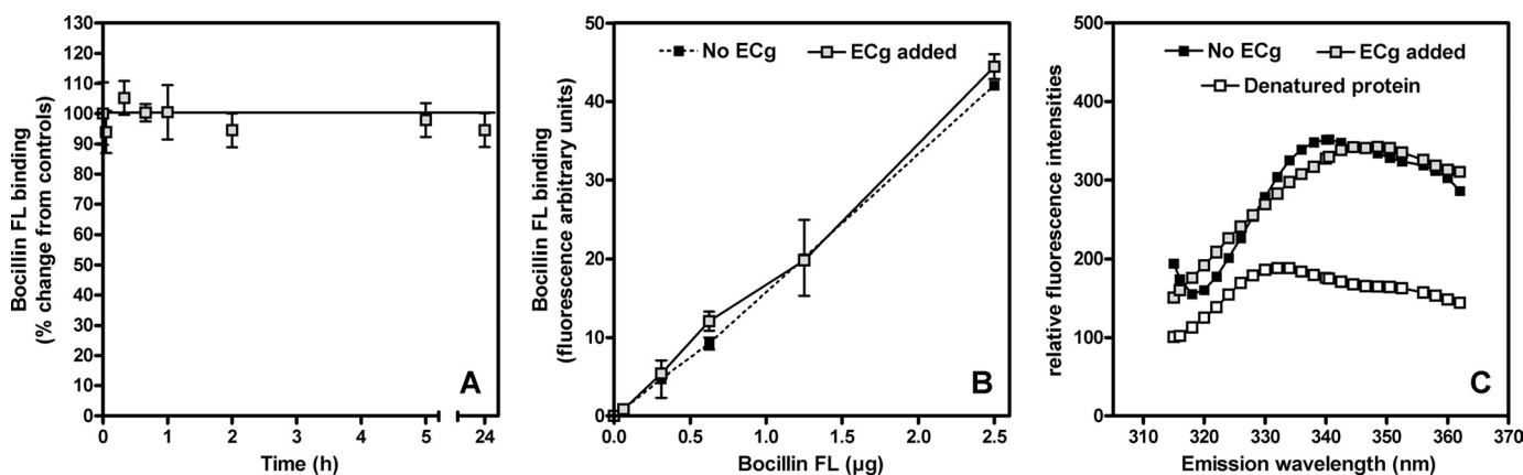
FIGURE 5. \beta -Lactam binding (A and B) and fluorescence assay (C) of PBP2a in 25 mM HEPES, 1 M NaCl (pH 7.0). A, binding of the fluorescent penicillin derivative Bocillin FL to PBP2a (5 \mu\text{M} ). PBP2a was incubated for up to 24 h in 12.5 \mu\text{g}/\text{ml} ECg. The samples were then incubated for 25 min in the presence of 1.25 \mu\text{g} of Bocillin FL and prepared for fluorescence measurement. The results were expressed as percentages of change from controls (no ECg added). The values are the means \pm S.D. B, binding of increasing concentrations of Bocillin FL to PBP2a (5 \mu\text{M} ). PBP2a was incubated over 1 h in 12.5 \mu\text{g}/\text{ml} ECg. Binding was then measured after 25 min in the presence of increasing concentrations of Bocillin FL. The values are the means \pm S.D. C, tryptophan fluorescence emission spectra of PBP2a (0.18 \mu\text{g}/\text{ml} ). The pretreatments of PBP2a are as follows: ECg added (1 h, 12.5 \mu\text{g}/\text{ml} ) and denatured protein (1 h, 60 ^{\circ}\text{C} ). We have previously determined (36) that the Bocillin FL concentrations employed in these experiments enable the detection of changes in the affinity of PBP2a for \beta -lactam antibiotics.
