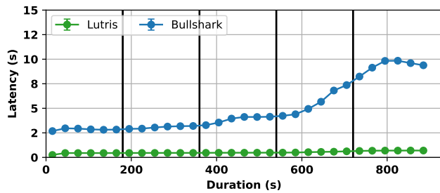
Figure 7: Performance of a 10-validators committee when up to 3 validators crash and recover.
