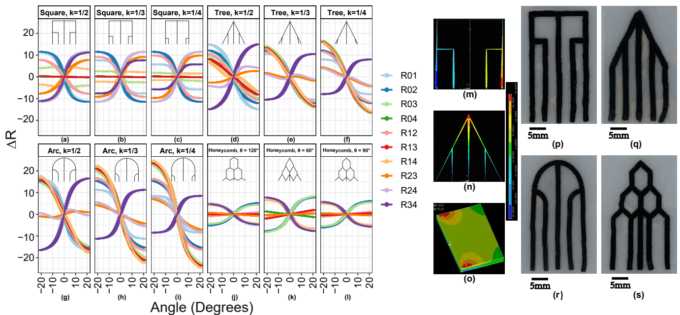
Fig. 5: Resistance Variations Analysis in Proposed Patterns Under Horizontal Bending: (a-c) Square-Like Pattern, (d-f) Tree-Like Pattern, (g-i) Arc-Like Pattern, (j-l) Honeycomb-Like Pattern. (m-o) Simulations of (m) Square-Like Pattern, (n) Tree-Like Pattern, and (o) Horizontal Bending with a Sensor (Unit: N). (p-s) Four Multi-DoF Sensing Patterns After Fabrication
