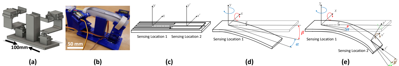
Fig. 6: (a) The 3D Model of Test Setup. (b) Real Testing photo of the Finger-like Test Setup. (c-e) Schematic diagrams illustrating the test setup: (c) Simplified view with the sensor positioned on top. (d) Deformation in locations 1. (e) Deformation in both locations 1 and 2.
