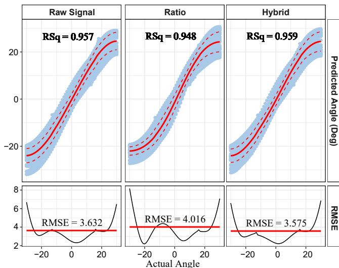
Fig. 7: Model Comparison for Sensing Location 1 in Horizontal Bending: Top plots show model-predicted vs. actual angles; bottom plots display RMSE variations vs. actual angles.
