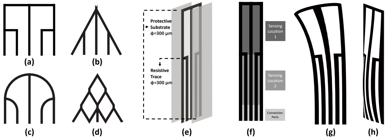
Fig. 1: (a-d) Four multi-DoF trace designs. (e) Overview of sensor layers layout. (f) Detailed view of sensing locations and connection parts. (g) Lateral bending in Sensing Locations 1. (h) Vertical bending in Sensing Locations 2.
