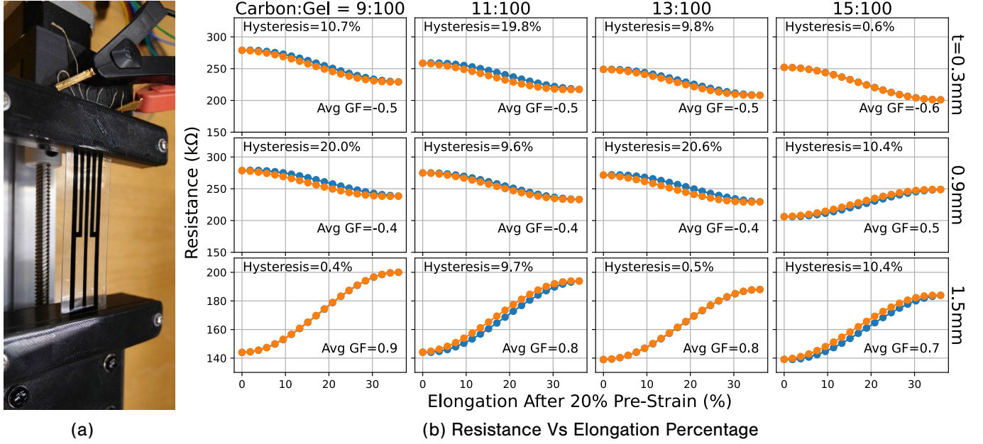
Fig. 4: (a) Stretching test setup: sample clamping and measurement are shown. (b) Resistance Variation with Elongation Percentage for Different Carbon-Gel Weight Ratios and Conductive Layer Thicknesses. The maximum hysteresis and gauge factor (GF) are indicated at each subplot's top left and bottom right.
