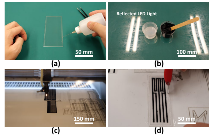
Fig. 2: (a) A 300 \mu\text{m} acrylic sheet, laser-cut into a frame, is glued onto a 2000 \mu\text{m} acrylic base to create the molding frame. (b) Preparation of the Platsil mixture (left) for combination with the carbon-isopropyl alcohol mixture (right). (c) Laser-cutting of the cured conductive substrates to form conductive traces. (d) The final sensors were sealed with non-conductive Platsil mixtures on both sides, followed by demolding.
