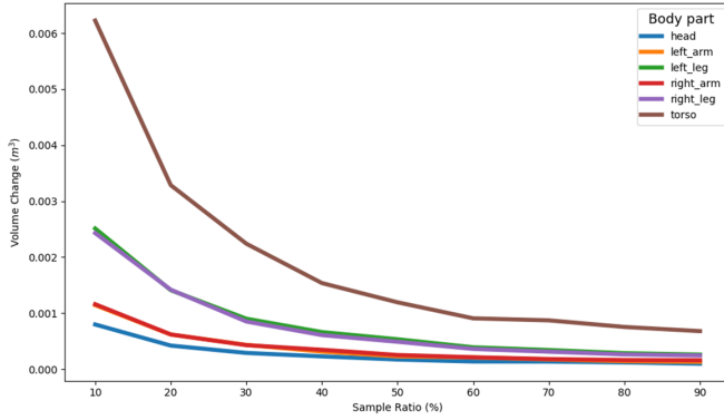
Fig. 10. Measured volume change against input scale changes.
