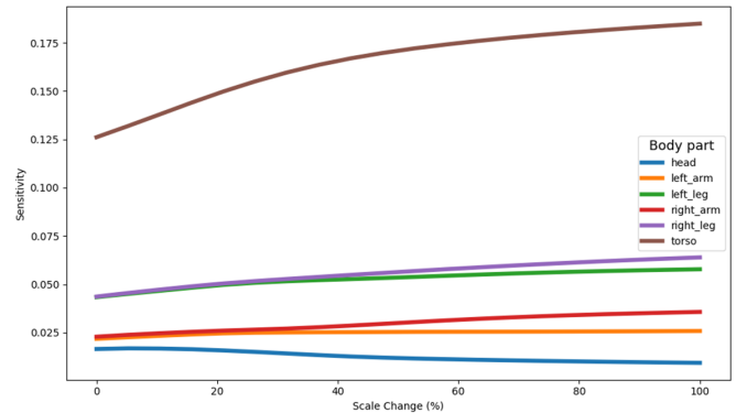
Fig. 9. Graph of \frac{\overline{\Delta V}}{\Delta X} (sensitivity) against input scale.
