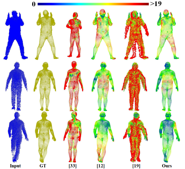
Fig. 7. Comparison of shape reconstruction error with related works. Each point is colored based on the per-vertex error in millimeters.
