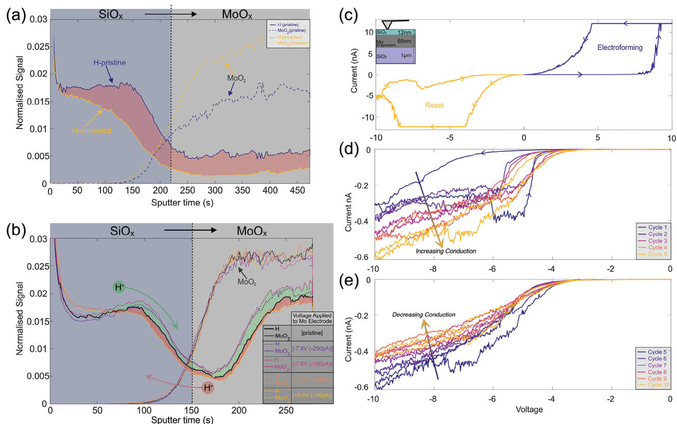
Figure 4. a) SIMS depth profiles normalized to the total ion signal for pristine HSQ \text{SiO}_x samples before and after annealing revealing a loss of hydrogen during annealing. IBA analysis of the annealed sample (sample 6) is shown in Figure S4 (Supporting Information). b) SIMS depth profiles normalized to the total ion signal comparing the hydrogen concentration in sample 4 between pristine devices as well as devices electrically biased with opposite polarities. Increases and decreases in the hydrogen concentration at each depth are illustrated with green and red shading, respectively. This illustrates the reversible field-driven diffusion of hydrogen to and from the interface under negative and positive voltages applied to the bottom electrode. Corresponding IBA analysis is found in Figure S2 (Supporting Information). Forward and reverse IV sweeps carried out on a comparable \text{SiO}_x sample to that in b) show: c) electroforming and resetting, d) an initial increase in conduction from cycles 1–5 with a negative bottom electrode bias, e) a decrease in conduction under the same bias from cycles 5–10.
