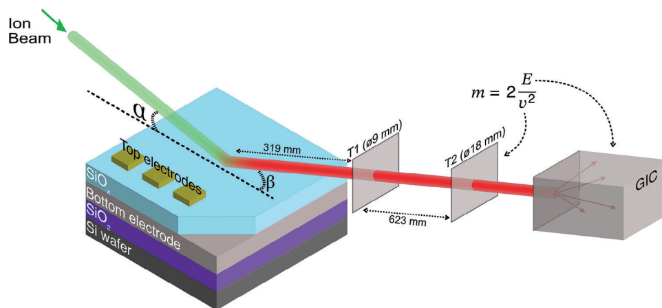
Figure 1. Schematic of the samples and the ToF-ERDA analysis applied at the University of Jyväskylä, \alpha/\beta = 20.5^\circ . The ion beam analysis is done in a clear region of SiO x , away from the Au/Ti top electrodes to prevent interference. A high energy (MeV) beam of primary ions (green beam) is used to irradiate the sample surface at a glancing angle, \alpha . This elastically forward recoils sample atoms (red beam) at angle \beta into two timing detectors and a gas ionization chamber, which measure the speed and energy of the atoms, respectively. This enables the determination of the element ejected and its original depth within the material.
