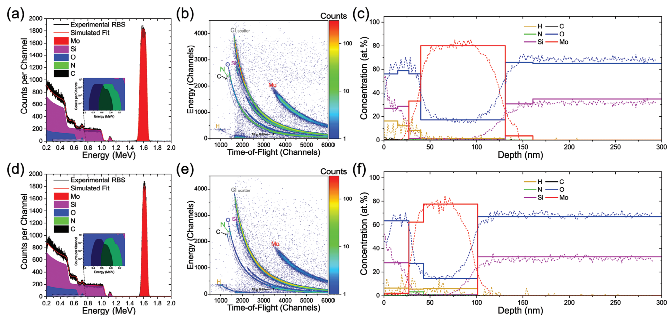
Figure 2. IBA measurements of two samples with nominally the same composition, with a similar thickness of \text{SiO}_x deposited using a)–c) Sample 1 – ALD and d)–e) Sample 9 – Sputtering, onto Mo bottom electrodes. a,d) RBS spectra for the sample confirm the concentration of heavier elements. b,e) ToF-ERDA spectra for both samples, used to generate initial depth profiles (dotted lines) in (c,f). For these depth profiles, concentrations of heavier elements are generated from the beam scatter and are not as accurate due to extended tails from measurement artefacts such as multiple scattering. The solid lines in (c,f) show the final sample composition generated by fitting the ToF-ERDA results from MCERD to RBS measurements, giving a reliable measure of composition for the full range of elements. For both samples, significant concentrations of H, C, and N impurities were measured, along with oxidation of the Mo electrodes.
