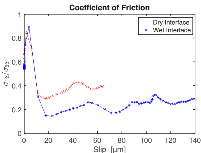
Fig. 9. Evolution of friction with slip along a dry (red) and prewetted (blue) interface. Friction is obtained as the ratio of shear to normal stress measured using the ultrahigh-speed DIC method over a field of view of size 18 \times 11 mm 2 . The curves are obtained for a point at the center of the field of view, with other locations showing similar behavior. The two tests are conducted under the same nominal loading conditions of P = 15 MPa and \alpha = 29^\circ . In these tests, ruptures are initiated by using a different procedure, not involving fluid injection (as described in Dynamic Friction Measurements for Dry versus Wet Interfaces using Ultrahigh-Speed DIC ), so as to better characterize the role of preexisting fluids on the interface.
