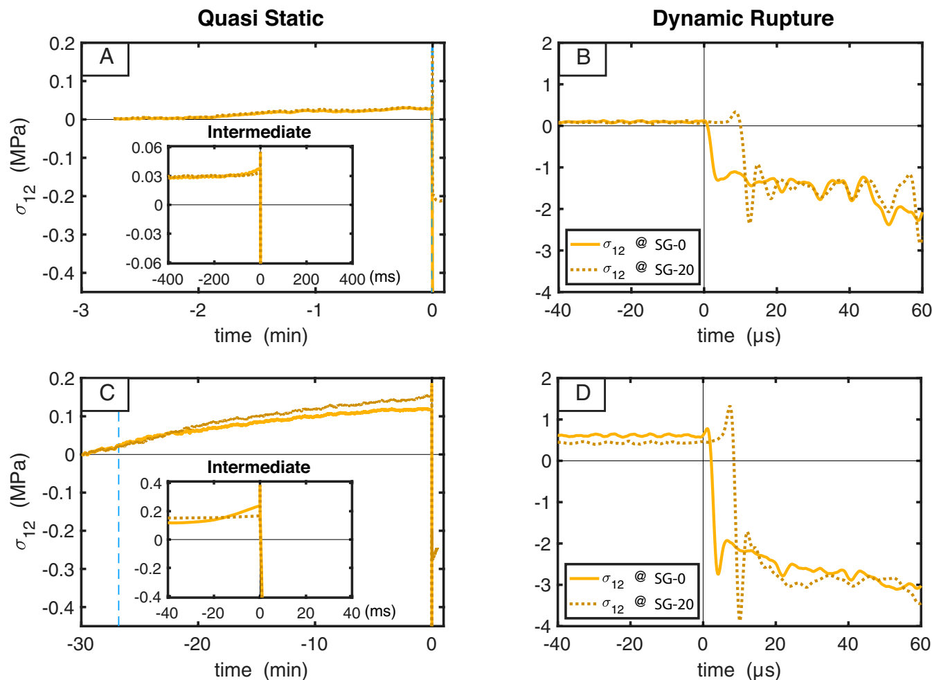
Fig. 7. Shear-stress evolution from the two strain gauges SG-0 and SG-20 (Fig. 2B and SI Appendix , Fig. S1B). The shear stress \sigma_{12} is shown over three time scales: minutes (A and C), milliseconds (A, Inset , and C, Inset ; notice the different scales of both axes), and microseconds (B and D). t = 0 corresponds to the rupture initiation. (A) Shear stress during rapid pressure ramp-up in the few minutes prior to the opening of the solenoid valve. No fluid has been delivered to the interface yet, and \sigma_{12} accumulates as a consequence of the viscoelastic relaxation of the bulk polymer under constant external load. Upon the opening of the valve, in the few hundred milliseconds prior to the rupture initiation (A, Inset ), there is minimal precursory stress redistribution due to limited accelerated slip prior to the incipient dynamic event. (B) Shear-stress evolution during the resulting (right-lateral) dynamic rupture. (C) Shear stress during slow pressure ramp-up. The delivery of pressurized fluid begins about 27 min prior to the rupture initiation, promoting heterogeneous slow slip and different \sigma_{12} variations from SG-0 to SG-20. Note that \sigma_{12} at both locations also accumulates as a consequence of the viscoelastic relaxation of PMMA. In the few tens of milliseconds leading to the rupture initiation (C, Inset ), \sigma_{12} redistributes due to the local accelerated slip at SG-0 as a precursor of the incipient dynamic event. (D) Shear-stress evolution during the resulting (right-lateral) dynamic rupture. Note that the stress drop is approximately twice as large as the one in the rapid ramp-up counterpart.
