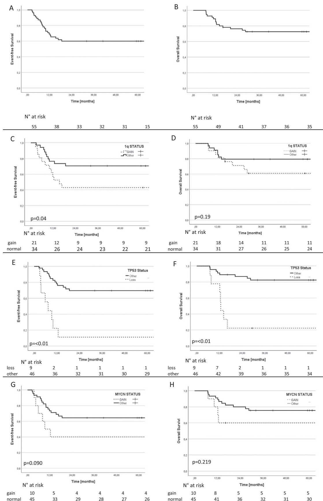
FIGURE 1 | Prognostic impact of the respective copy number variations (CNVs). A and B: all patients ( n = 55 ).
