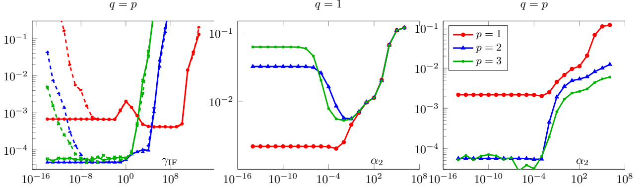
FIGURE 5.3. Dependence of the relative L^2 -error in B in terms of the choice of stabilization parameters. We consider a pure diffusion problem with (\mu_1, \mu_2) = (20, 2) in the geometry shown in Figure 5.1b. The solid lines in the left plot show the results for the method as defined and analyzed in this paper, while dashed lines display the results for an alternative method in which the term N_h^c in the bilinear form is omitted.
