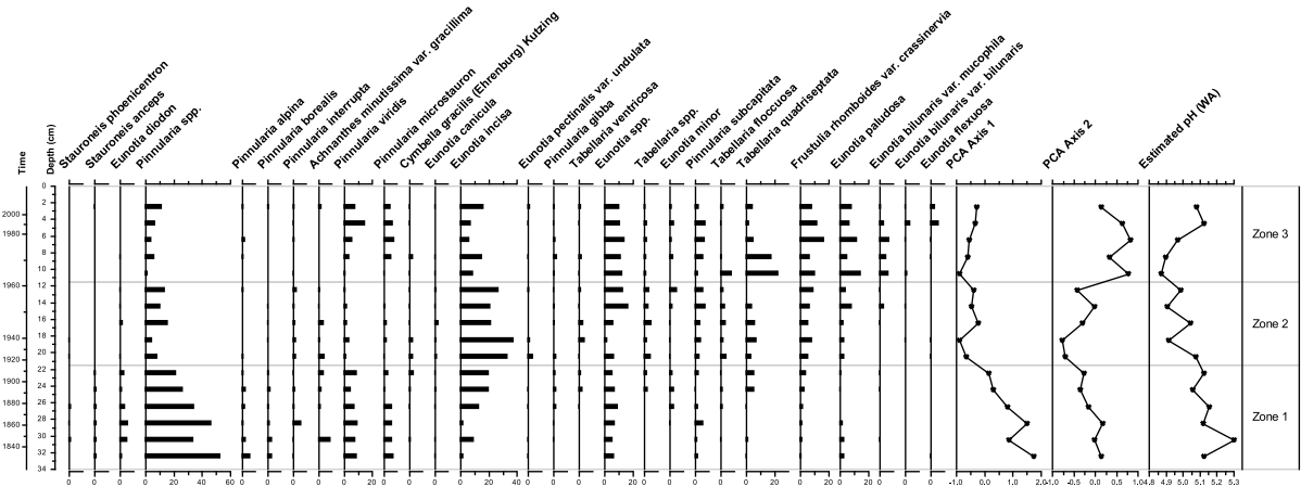
Fig. 3. Diatom plot for BGP1 with diatom species profiles expressed as percentage relative abundance. Also presented are PCA axis 1 & 2 values, transfer function reconstructed pH and characteristic zones derived from CONISS analysis.
