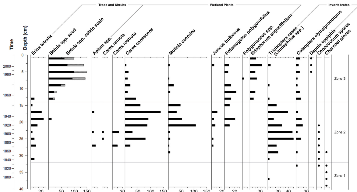
Fig. 4. Macrofossil plot for BGP1, expressed as number per 100 cm 3 of material. Zones designated by CONISS analysis shown on far right.
