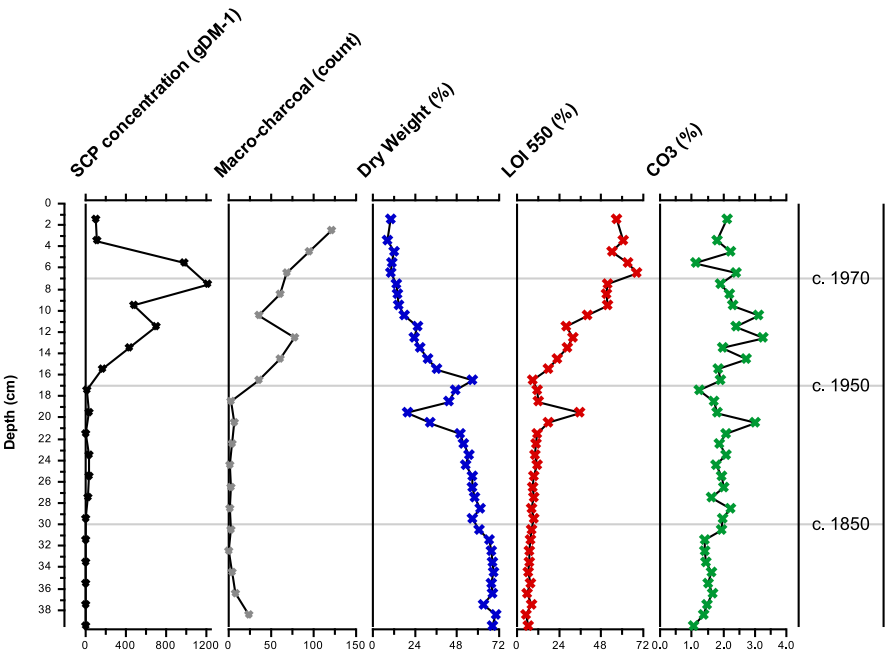
Fig. 2. SCP profile for BGP1 (black) and macro-charcoal profile (grey) plotted against core depth. Lithostratigraphic results for BGP1, showing dry weight (blue), loss on ignition (red) and carbonate (CO 3 ) (green). Horizontal lines correspond to approximate dates from SCPs.
