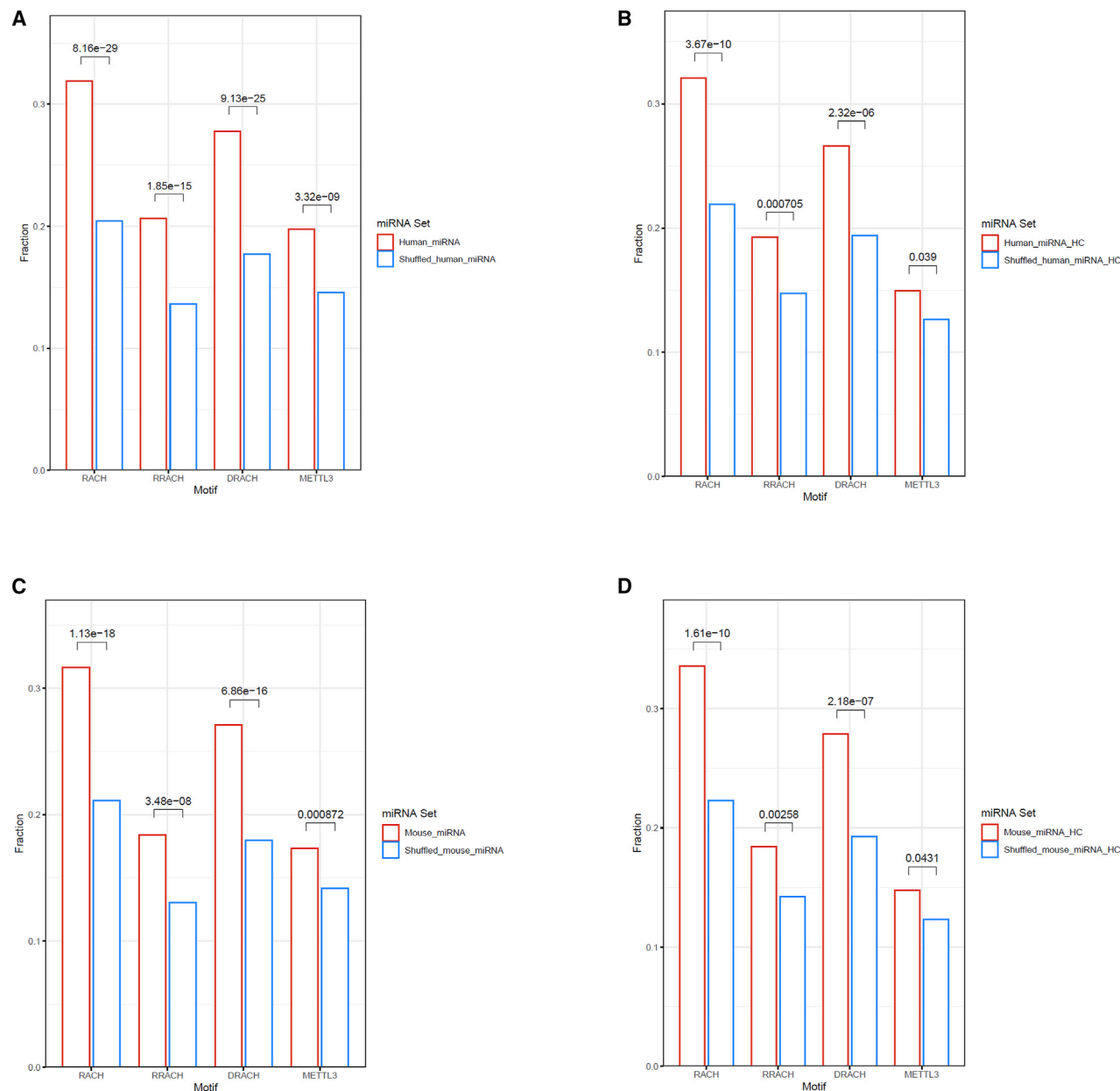
Figure 2. m6A consensus sequences in the human and murine miRNome
