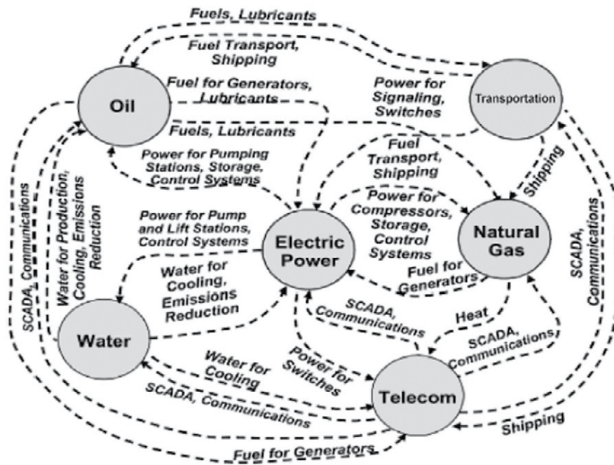
Figure 3: Examples of electric power infrastructure dependencies (Source: Rinaldi, 2001).
