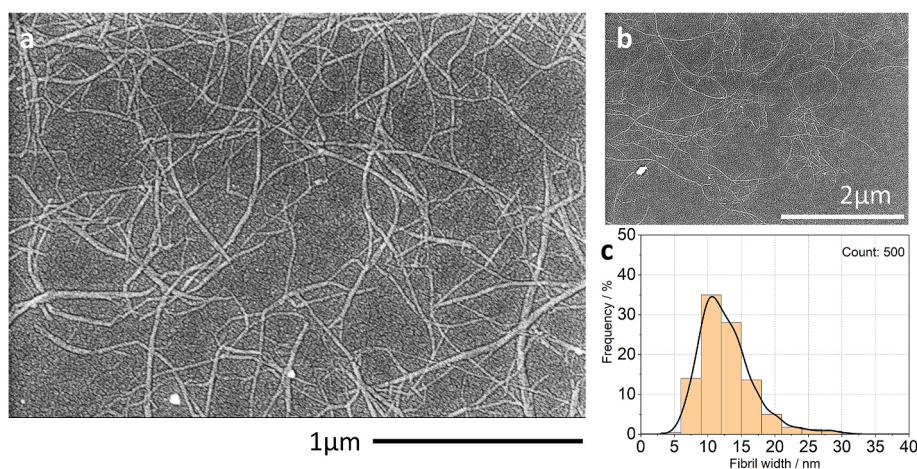
Fig. 6. FE-SEM images of nanofibrils from cow mature at (a) 45k and (b) 25k magnifications. (c) The fibril width distribution of cellulose nanofibrils.
