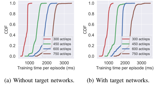
Figure 6: Cumulative distribution functions (CDFs) of training time per episode with different numbers of actions per episode.
