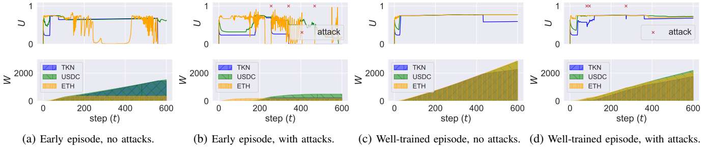
Figure 9: Utilization ratio ( U ) and reserve ( W ) of the RL environment's lending pools throughout each of the selected episodes. The red crosses ( \times ) in (b) and (d) indicate the steps ( t ) at which attacks occur.
