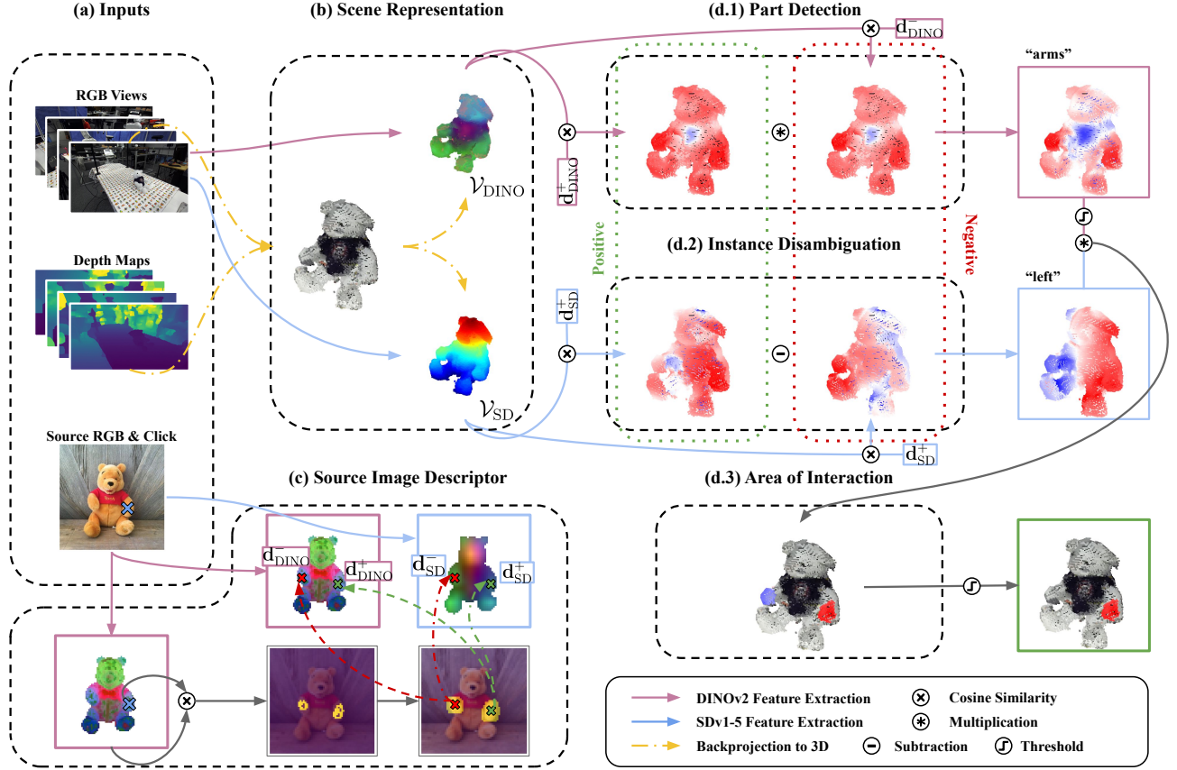
Fig. 2. Perception Modules \mathcal{O}_D , \mathcal{O}_G : (a) RGB-D images of the tabletop scene and a random source image of the object class are used as input, along with a single user-defined click, indicating the interaction area (Section III-A). (b) Images are lifted in 3D space by back-projection and interpolation of RGB values, densities, and features from DINO and SD (Section III-B). (c) DINO and SD features from the source image are extracted and used to localize instances of the user-defined part, automatically identifying them as positive (same instance type) or negative (different instance type), and extracting visual descriptors (Section III-C). (d) DINO descriptors localize corresponding parts in the 3D scene, while SD descriptors disambiguate between instances, resulting in a 3D mask identifying the proposed interaction area (Section III-D).
