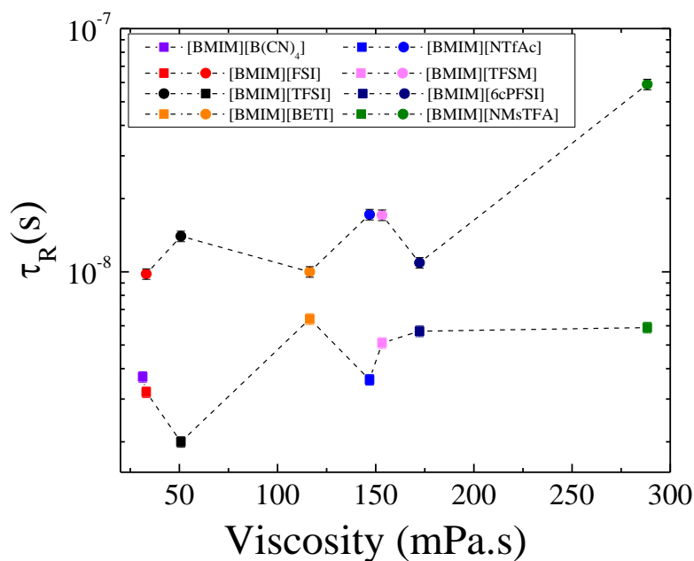
Figure 5. Average rotational time of [\text{BMIM}]^+ (squared symbols) and the corresponding anions (circular symbols) that contain ^{19}\text{F} in their chemical structures ( [\text{FSI}]^- , [\text{BETI}]^- , [\text{NTfAc}]^- , [\text{TFSM}]^- , [\text{6cPFSI}]^- and [\text{NMsTFA}]^- ) as a function of viscosity, at 25^\circ\text{C} . Viscosity values were taken with permission from reference (16). Rotational times of [\text{BMIM}]^+ and [\text{TFSI}]^- in [\text{BMIM}][\text{TFSI}] are included for comparison purposes and are taken with permission from reference (20). Dashed lines are guides to the eye.
