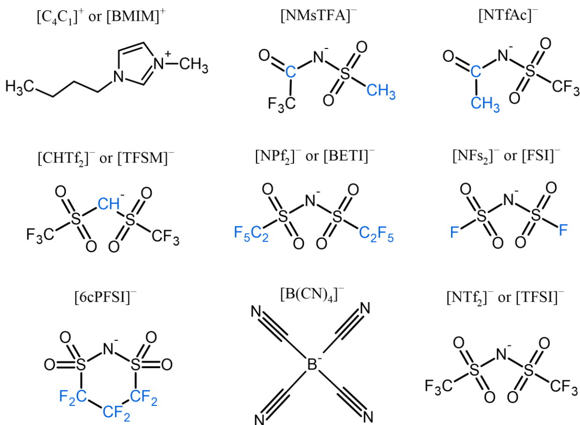
Figure 1. Molecular structure of the cation [\text{BMIM}]^+ and the anions of the studied ILs. The [\text{TFSI}]^- anion is included for comparison purposes and the chemical modifications in the anions are highlighted in blue color.
