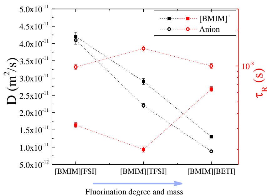
Figure 8. Diffusion coefficients (black symbols) and rotational times (red symbols) of [\text{BMIM}]^+ (squared solid symbols) and the corresponding anion (circular hollow symbols) in the three ILs of group C , at 25°C. Rotational times of [\text{BMIM}]^+ and [\text{TFSI}]^- in [\text{BMIM}][\text{TFSI}] are taken with permission from reference (20). Dashed lines are guides to the eye.
