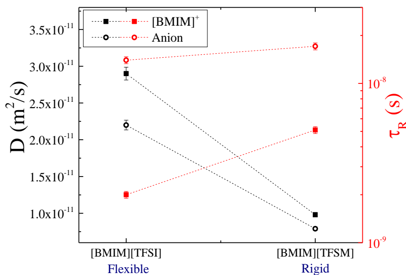
Figure 7. Diffusion coefficients (black symbols) and rotational times (red symbols) of [\text{BMIM}]^+ (squared solid symbols) and the corresponding anion (circular hollow symbols) in the ILs of group B , at 25°C. Rotational times of [\text{BMIM}]^+ and [\text{TFSI}]^- in [\text{BMIM}][\text{TFSI}] are taken with permission from reference (20). Dashed lines are guides to the eye.
