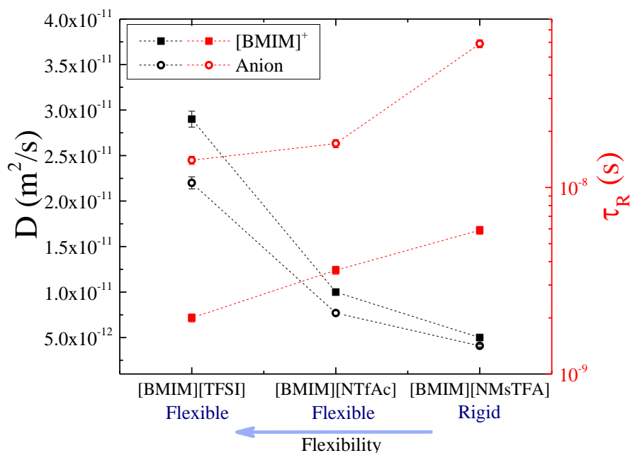
Figure 6. Diffusion coefficients (black symbols) and rotational times (red symbols) of [BMIM] + (squared solid symbols) and the corresponding anion (circular hollow symbols) in the three ILs of group A , at 25°C. Rotational times of [BMIM] + and [TFSI] − in [BMIM][TFSI] are taken with permission from reference (20). Dashed lines are guides to the eye.
