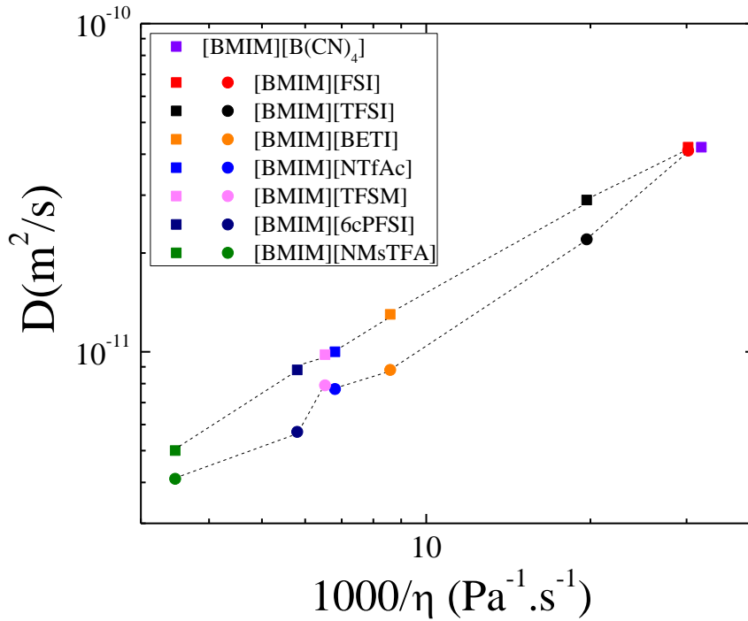
Figure 2. Diffusion coefficients of [\text{BMIM}]^+ (squared symbols) and the corresponding anion (circular symbols) as a function of fluidity (inverse of viscosity \eta ), at 25°C. Viscosity values were taken with permission from reference (16). Dashed lines are guides to the eye.
