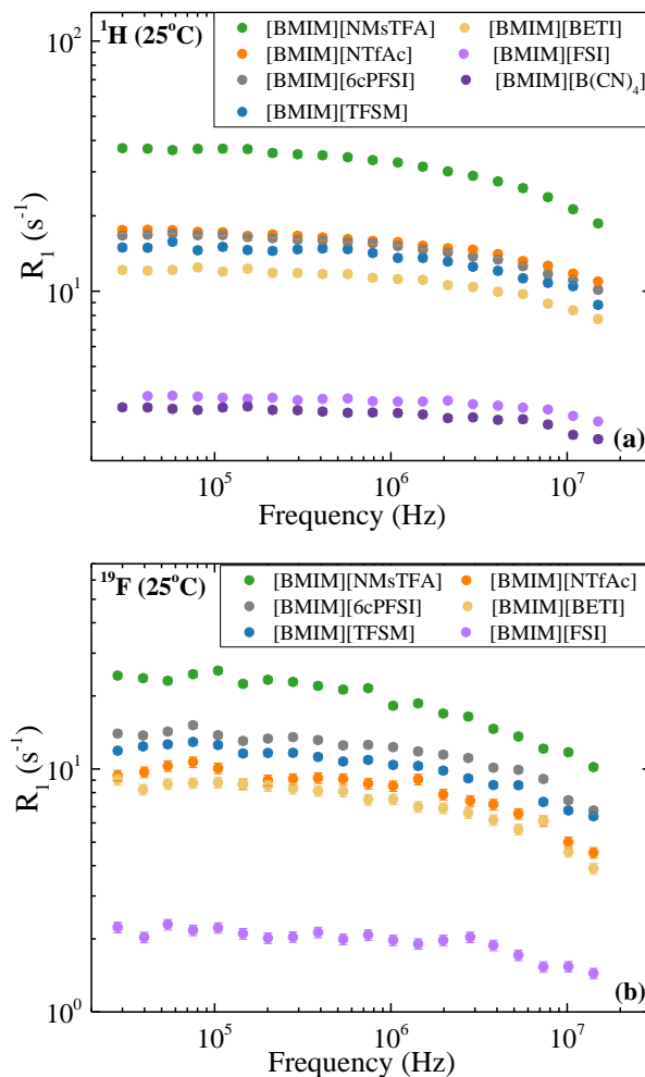
Figure 3. (a) ^1\text{H} ([BMIM] ^+ ) and (b) ^{19}\text{F} (anion) relaxation rate dispersions for [BMIM][NMSTFA], [BMIM][NTfAc], [BMIM][6cPFSI], [BMIM][TFSM], [BMIM][BETI], [BMIM][FSI] and [BMIM][B(CN) _4 ], at 25°C.
