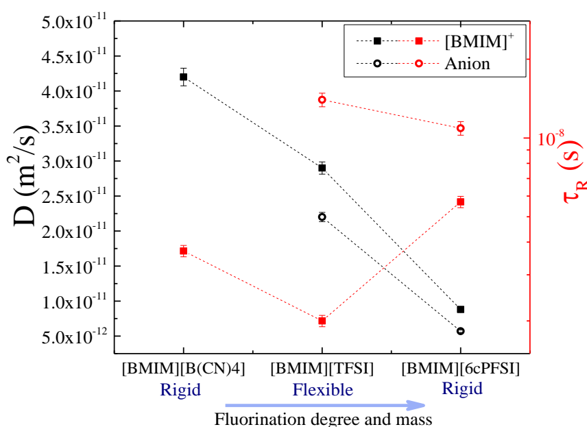
Figure 9. Diffusion coefficients (black symbols) and rotational times (red symbols) of [\text{BMIM}]^+ (squared solid symbols) and the corresponding anion (circular hollow symbols) in the three ILs of group D , at 25°C. Rotational times of [\text{BMIM}]^+ and [\text{TFSI}]^- in [\text{BMIM}][\text{TFSI}] are taken with permission from reference (20). Dashed lines are guides to the eye.
