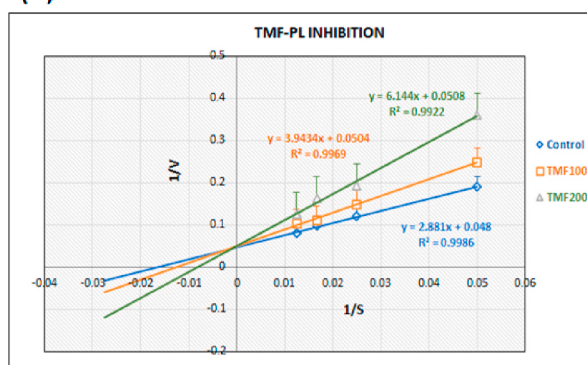
Fig. 3. Double reciprocal plots of PMF (A) and TMF (B), each at 100 and 200 \mu\text{g/mL} ( n = 3 biological repeats).
