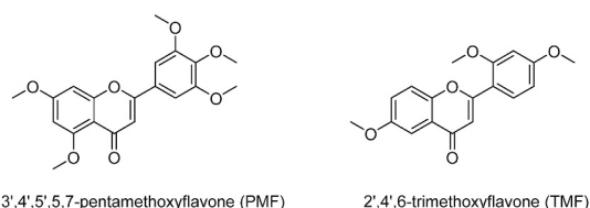
Fig. 1. Structures of PMF and TMF
