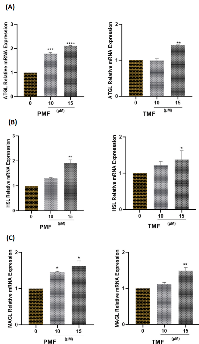
Fig. 13. Effects of PMF and TMF on lipolytic genes expression. (A) ATGL. (B) HSL. (C) MAGL. Data is represented as mean \pm SD ( n = 3 ). P^* < 0.05 , P^{**} < 0.01 , P^{***} < 0.001 , P^{****} < 0.0001 . Asterisks (*) represent significant difference from the control.
