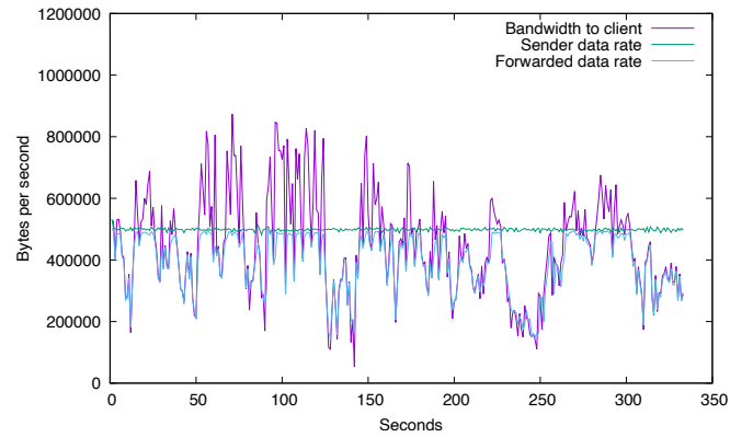
Fig. 3: Flow rates with Threshold Relaxation of 1
