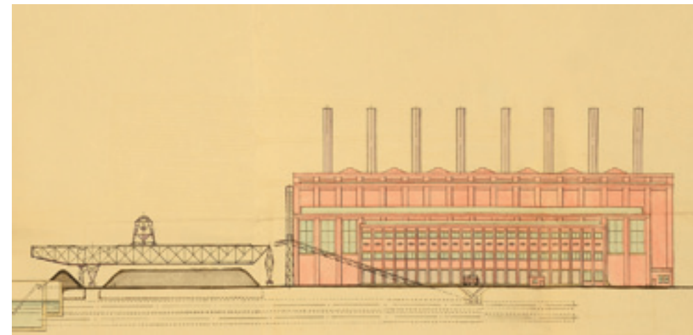
419. Battersea Power Station, proposed west elevation to Station 'A' from the first design by S. L. Pearce, engineer, 1927
