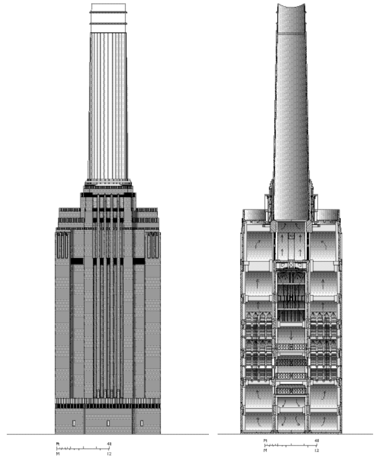
422. Battersea Power Station, elevation and section of typical corner tower and chimney as built
