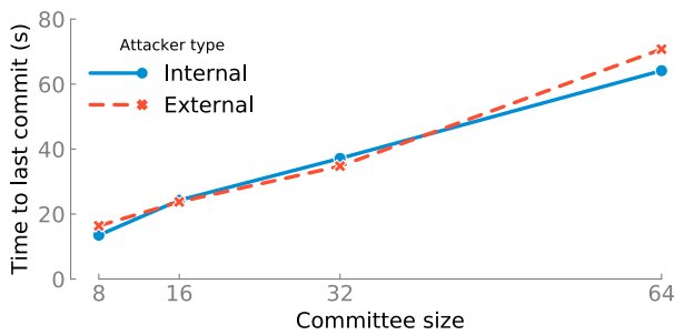
Figure 8: Unpredictable leader-tracking attacks.
