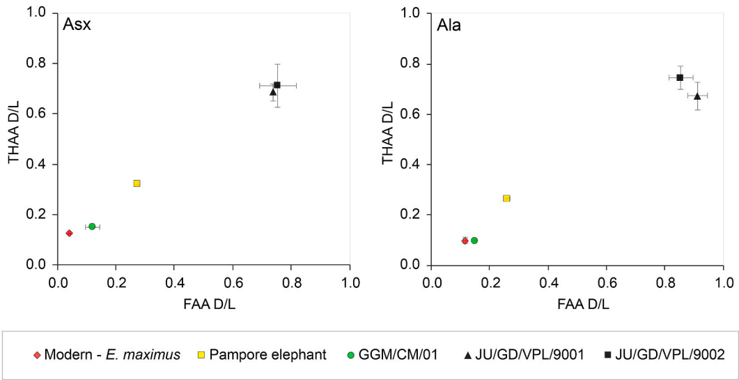
Fig. 6. Comparison two different amino acid (FAA) vs. total hydrolysable amino acid (THAA) intra-crystalline racemisation in the proboscidean enamel from the Jammu and Kashmir region for two different amino acids: Asx (left) and Ala (Right). Modern Elephas maximus enamel has been included for comparison (data from Dickinson et al., 2019). GGM/CM/01: Elephas cf. maximus , River Terrace T1, immediately above the Upper Siwalik Boulder Conglomerate; JU/GD/VPL/9001: Elephas planifrons , mudstone horizon underlying volcanic ash bed in Pinjor Formation; JU/GD/VPL/9002: Stegodon cf. insignis , mudstone horizon underlying volcanic ash bed in Pinjor Formation. Error bars depict 1σ about the mean based on replicate sub-samples.
