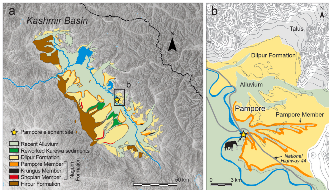
Fig. 3. Geological map of the Kashmir Valley (a) and the area around Pampore (b). The elephant site is marked with a star and was found within the Pampore Member.
