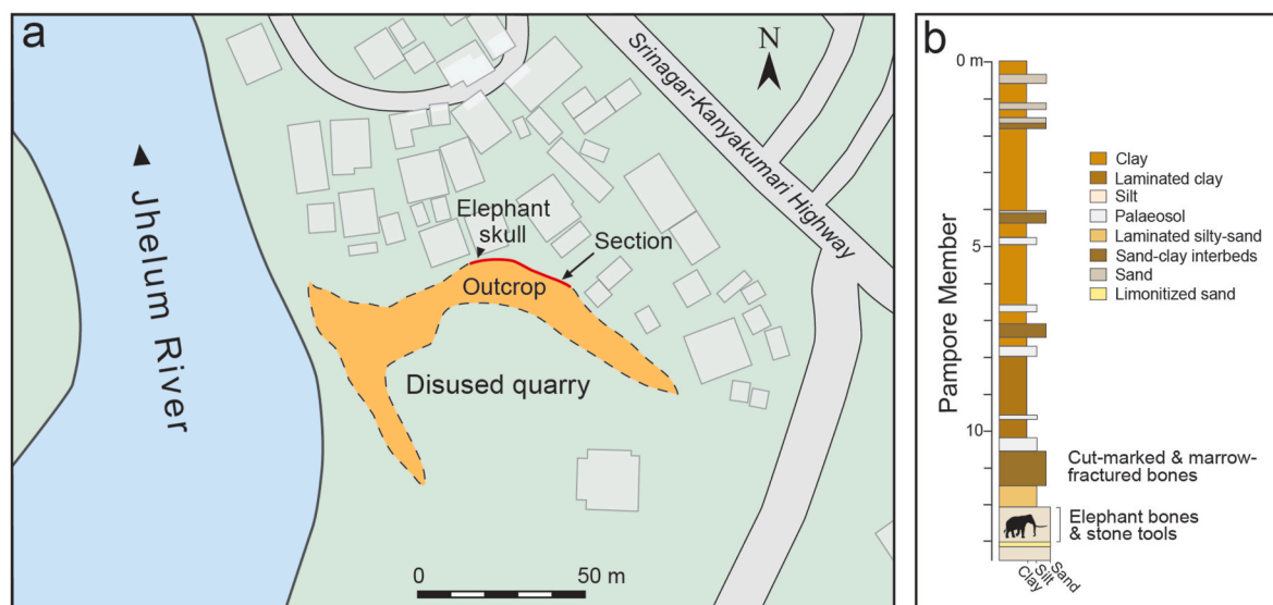
Fig. 4. Location of the Pampore Elephant site at Galander, near Pampore, with schematic section log through the sediments exposed in the outcrop.
