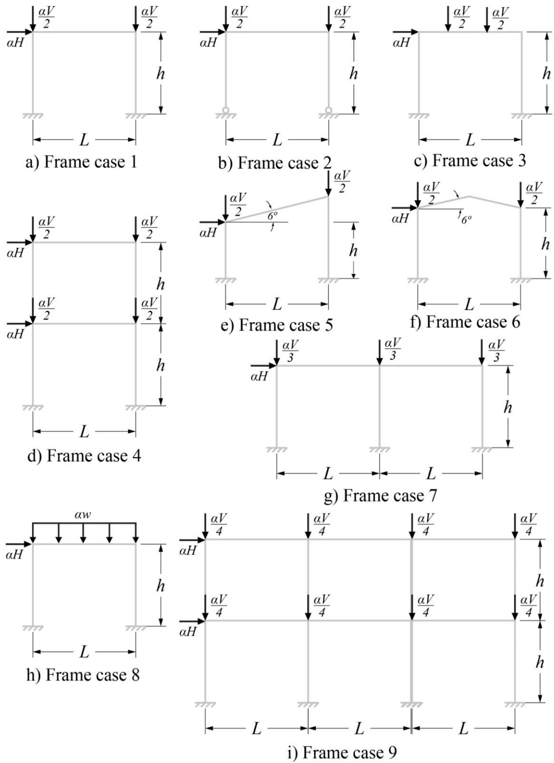
Figure 1: Details of modelled frames, where \alpha is the load factor.
