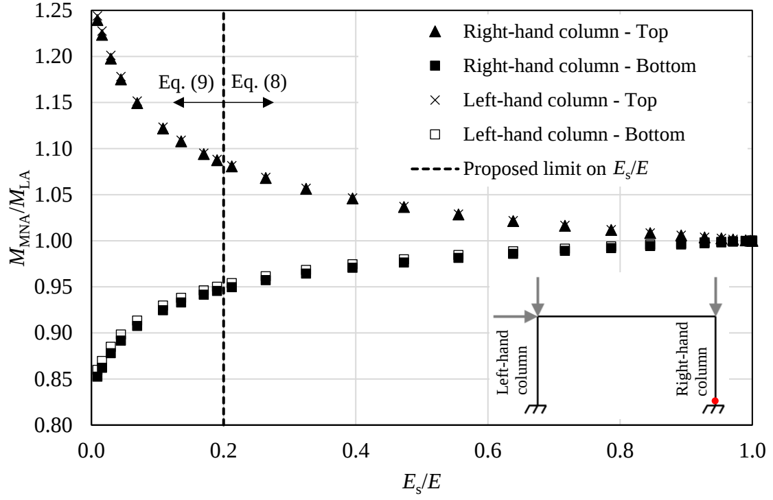
Figure 2: Ratio of internal moments obtained from a first order plastic ( M_{MNA} ) and elastic ( M_{LA} ) analysis at different locations in an example 5×10 m austenitic stainless steel portal frame plotted against the ratio of the secant modulus E_s to the elastic modulus E at the most heavily stressed point in the frame (as indicated by the red circle).
