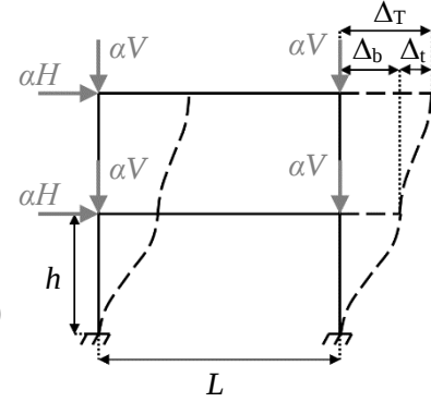
Figure 6: Example austenitic stainless steel two-storey frame where L=10 m and h=5 m and H=0.2V .
