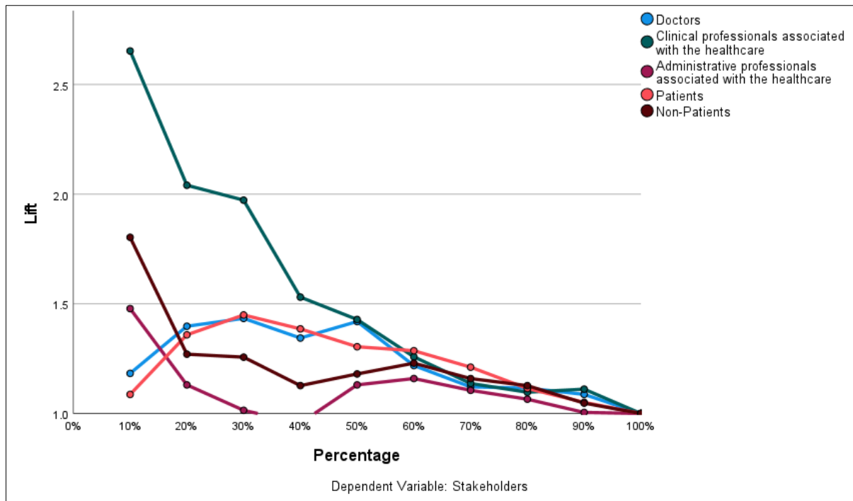
Figure 6: Lift Chart
