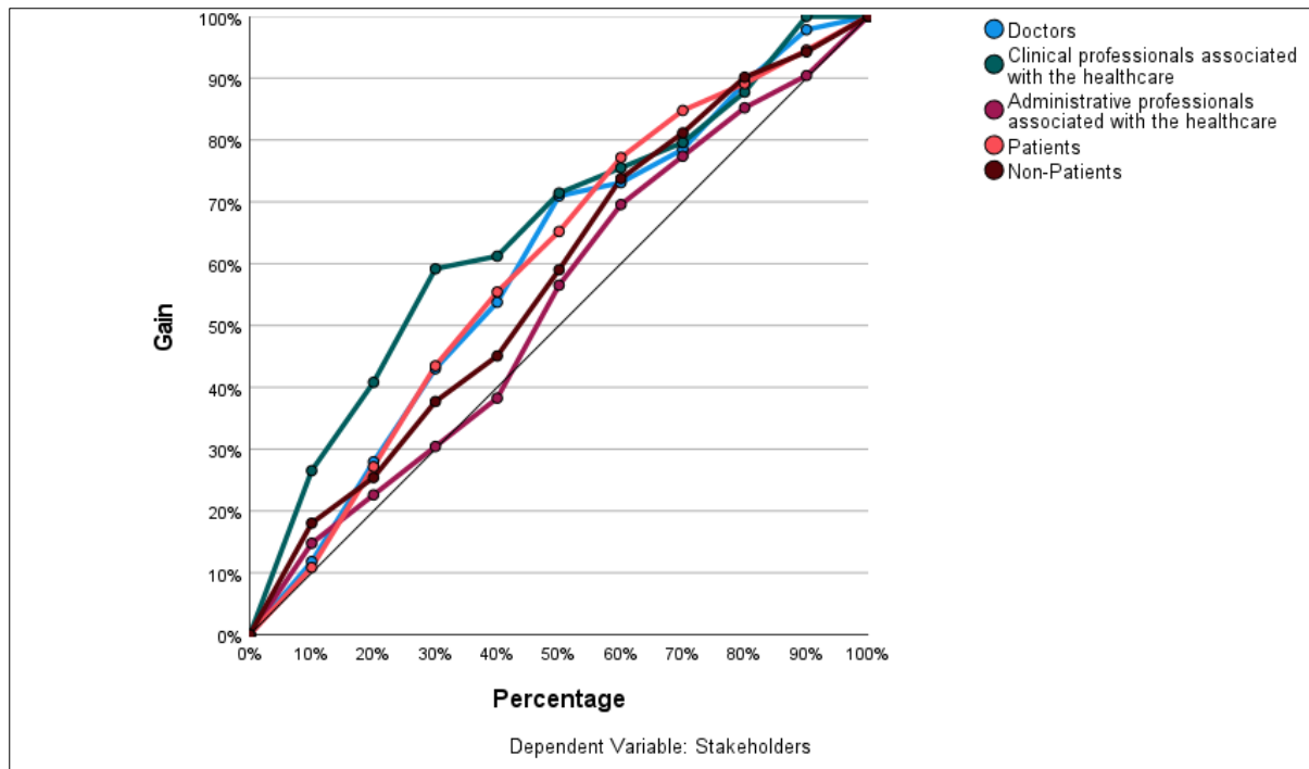
Figure 5: Gain Chart
