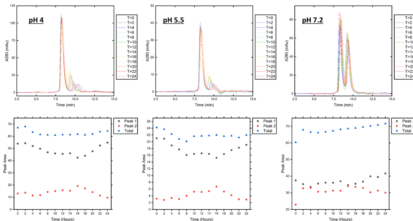
Fig. 8. HPLC SEC traces of LC-HN-VHH in the same solution conditions as used for the simulated pHs and ionic strengths (top). Integration of both peaks shows an inverse relationship of change in peak area over time, indicating a dynamic exchange of material from one elution peak to another, with little to no material loss (bottom).
