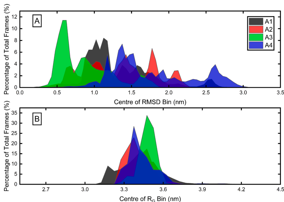
Fig. 3. A: Whole protein RMSD distribution after fixing the LC-H N domains, in bins of 0.05 nm width, all pH combined, with respect to its starting position for each model. B: R_G distribution in bins of 0.05 nm width, all pH combined. This shows the large overlap of values from all starting positions, with A3 maintaining a lower RMSD than other starting models.
