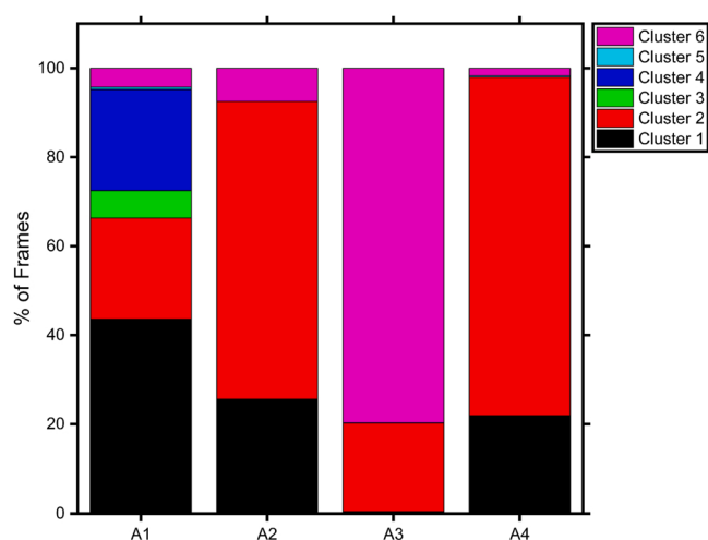
Fig. 5. Clustering of the frames, represented as a percentage of the total number of frames for each starting model. Reveals two clusters which exist in all models (2 and 6), with cluster 2 dominating the overall distribution and cluster 6 dominating in model A3.
