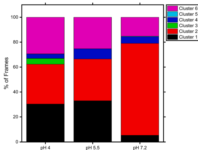
Fig. 9. Cluster distribution as a function of pH shows most frames in pH 7.2 are in cluster 2; while pH 4 and 5.5 have an almost equal proportion of frames in clusters 1, 2 and 6.
