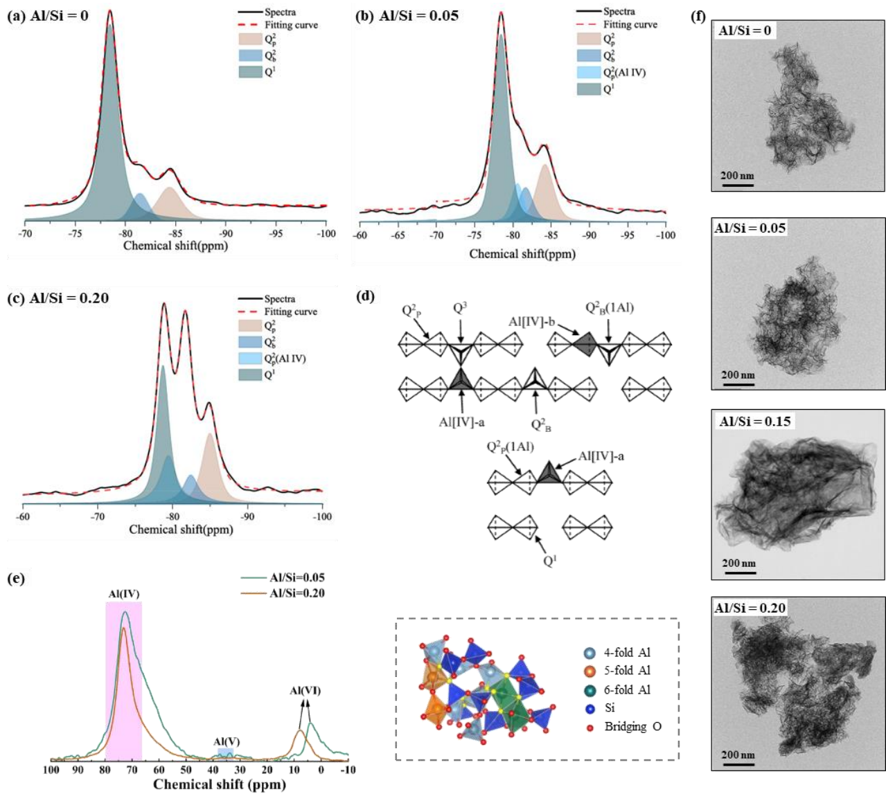
Fig. 9. ^{29}\text{Si} NMR spectra of (a) C-S-H and C-A-S-H with (b) Al/Si=0.05 and (c) Al/Si=0.20, with (d) Deconvolution based on aluminosilicate chains in C-A-S-H; (e) ^{27}\text{Al} NMR spectra of C-A-S-H with different Al/Si ratios and (f) Corresponding TEM images (Adapted from Refs. [131, 133, 138, 142]).
