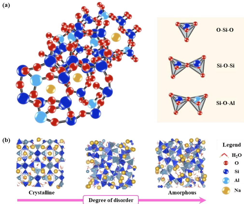
Fig. 3. Nanostructure of N-A-S-H regarding (a) 3D view, and (b) simulation from crystalline to amorphous N-A-S-H with Si/Al \approx 1.5 (Adapted from Refs. [64, 69]).
