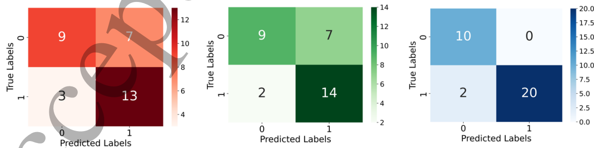
Figure 7. Confusion matrices for logistic regression (left), SVM (middle), DNN (right) models on the test dataset (pristine = 1, aged = 0).
