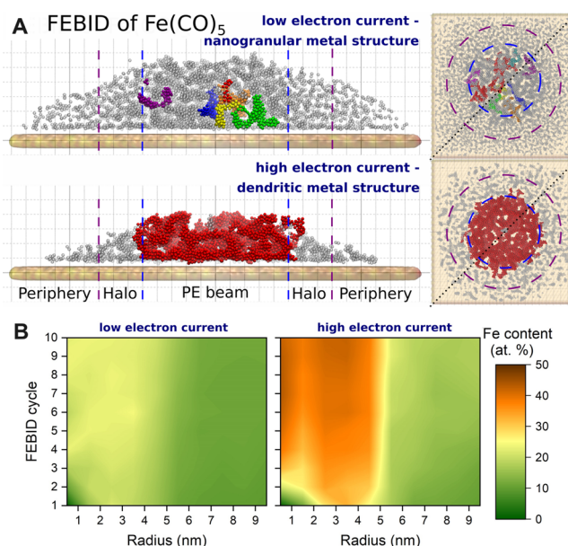
Figure 25. Results of the IDMD simulations 54 of the FEBID process for \text{Fe}(\text{CO})_5 . (a) Snapshots of the simulated iron-containing nanostructures: side view on diagonal cross sections indicated by dotted lines (left) and top view (right). The top and bottom snapshots in panel (a) correspond to electron currents of 1 and 4 nA, respectively. Only iron atoms are shown for clarity. Topologically disconnected metal clusters containing more than 100 iron atoms are shown in different colors. Smaller clusters containing less than 100 iron atoms are shown in gray. Boundaries of the primary electron beam, halo, and peripheral regions are indicated by dashed lines in the left column and by circles in the right column. Grid line spacing is equal to 1 nm in all dimensions. (b) Atomic Fe content of the grown iron-containing structures as a function of the number of simulated irradiation-replenishment FEBID cycles for electron currents of 1 (left) and 4 nA (right). Adapted with permission from ref 54. Copyright 2022 Royal Society of Chemistry.
