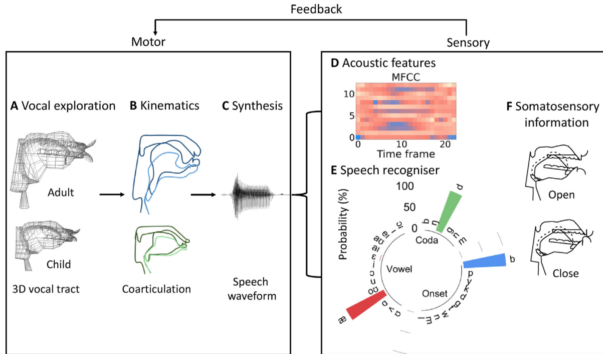
Fig. 1. Schematic overview of the steps involved each time the model tries a new set of articulatory targets (A) The adult vocal tract model is based on the MRI data of an adult male speaker and the child vocal models are scaled versions of the adult model (Birkholz & Kröger, 2007; Davis & Mermelstein, 1980; Goldstein, 1980). (B) Context-sensitive articulator kinematic movements are calculated by a synchronised dimension-specific sequential target approximation model (Liu et al., 2022; Xu, 2020). (C) Aero-acoustic simulation is based on enhanced area functions of time-varying vocal tract shapes to generate speech. (D) Mel-frequency cepstral coefficients (MFCCs) (Davis & Mermelstein, 1980) of natural and synthetic words were extracted. (E) A speech recogniser evaluates the probability of the targeted onset consonant, vowel and coda consonant, as represented by International Phonetic Alphabet (IPA) symbols. (F) Somatosensory information for limiting vocal exploration, provided by the cross-sectional areas to determine whether there is a closure in the vocal tract.
