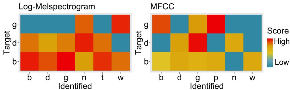
Fig. A2. Confusion matrices of consonants trained by MFCCs and Log Mel spectrograms, evaluated by a word recogniser. The score shows the weighted negative log likelihood loss. Higher scores represent higher phoneme probability. The bilabial stops trained by Log Mel spectrograms had fairly high accuracies, while the alveolar stops trained by MFCCs had higher accuracies. However, the velar stops trained by Log Mel spectrograms were identified as /n/ or /w/. Overall, the speech trained by Log Mel spectrograms were slightly better identified than that trained by MFCCs.
