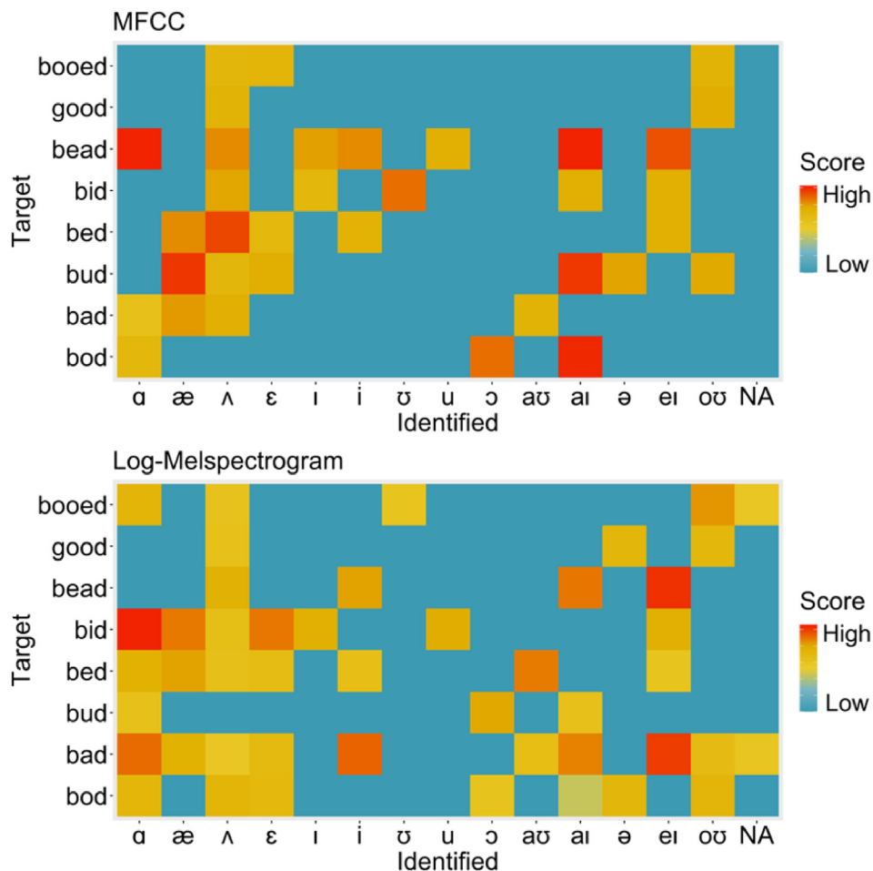
Fig. A3. Confusion matrices of vowels trained by MFCCs and Log Mel spectrograms, evaluated by a word recogniser. The score shows the weighted negative log likelihood loss. Higher scores represent higher phoneme probability. The recognition accuracies were higher for vowels trained by MFCCs than the ones trained by Log Mel spectrograms. Both acoustic features failed to guide the learning of intelligible vowels in 'booed' and 'good'. For the rest of the vowel categories, those trained by MFCCs were identified more correctly than the ones trained by Log Mel spectrograms. Especially, the vowel in 'bud' was less successful when trained by Log Mel spectrograms.
