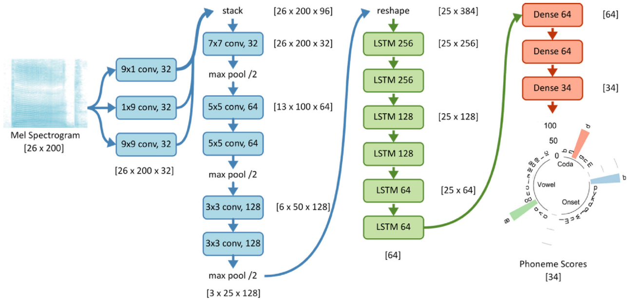
Fig. A4. Schematic diagram of the speech recogniser. The network contains 8 convolutional layers (conv), 6 long short-term memory (LSTM) layers and 3 dense layers (Dense). Batch normalisation layers after each conv, LSTM and Dense layers and dropout layers after each LSTM and Dense layers are not shown in the diagram. The architecture consists of 3 main parts: spectrotemporal feature processing, temporal feature processing and classification. The first convolutional layer module (in blue) was designed to learn the feature representations that may coexist or correlate in the spectral and temporal domains. The temporal feature processing module (in green) was designed to learn the temporal dependency and/or the state-based behaviour of the feature. Lastly, the classification module (in red) was used to learn the relationship between the features for classifying phonemes.
