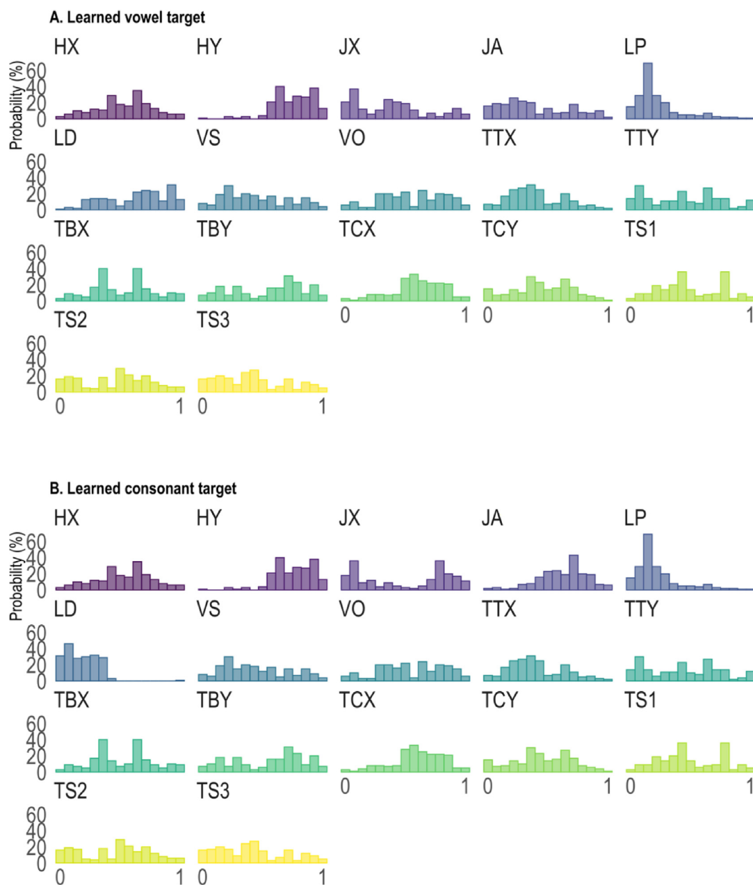
Fig. 10. Learned vocal tract parameters of syllabic cV and cV targets after the optimisation of the CV sequence in 'bad'. Histograms show 200 sets of learned targets with lowest recognition errors for the syllabic cV and cV target separately. For the cV target, tongue tip and tongue body horizontal positions (TCX, TTX), hyoid height (HY), lip protrusion (LP) exhibit concentrated distribution, while jaw angle (JA), jaw horizontal position (JX) lip distance (LD) seem widely distributed. The cV controlled LD, JA and JX during coarticulation and these parameters are narrowly distributed after training.
