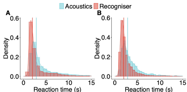
Fig. 7. Effects of type of auditory feedback on simulated vocal learning. (A, B) Reaction time of American English listeners in the open-vocabulary dictation task (A) and in the multiple-choice task (B). The vertical lines represent the median reaction time for the two types of auditory feedback. The listeners were asked to identify CVC and CVCV words learned by vocal tract models of different ages.
