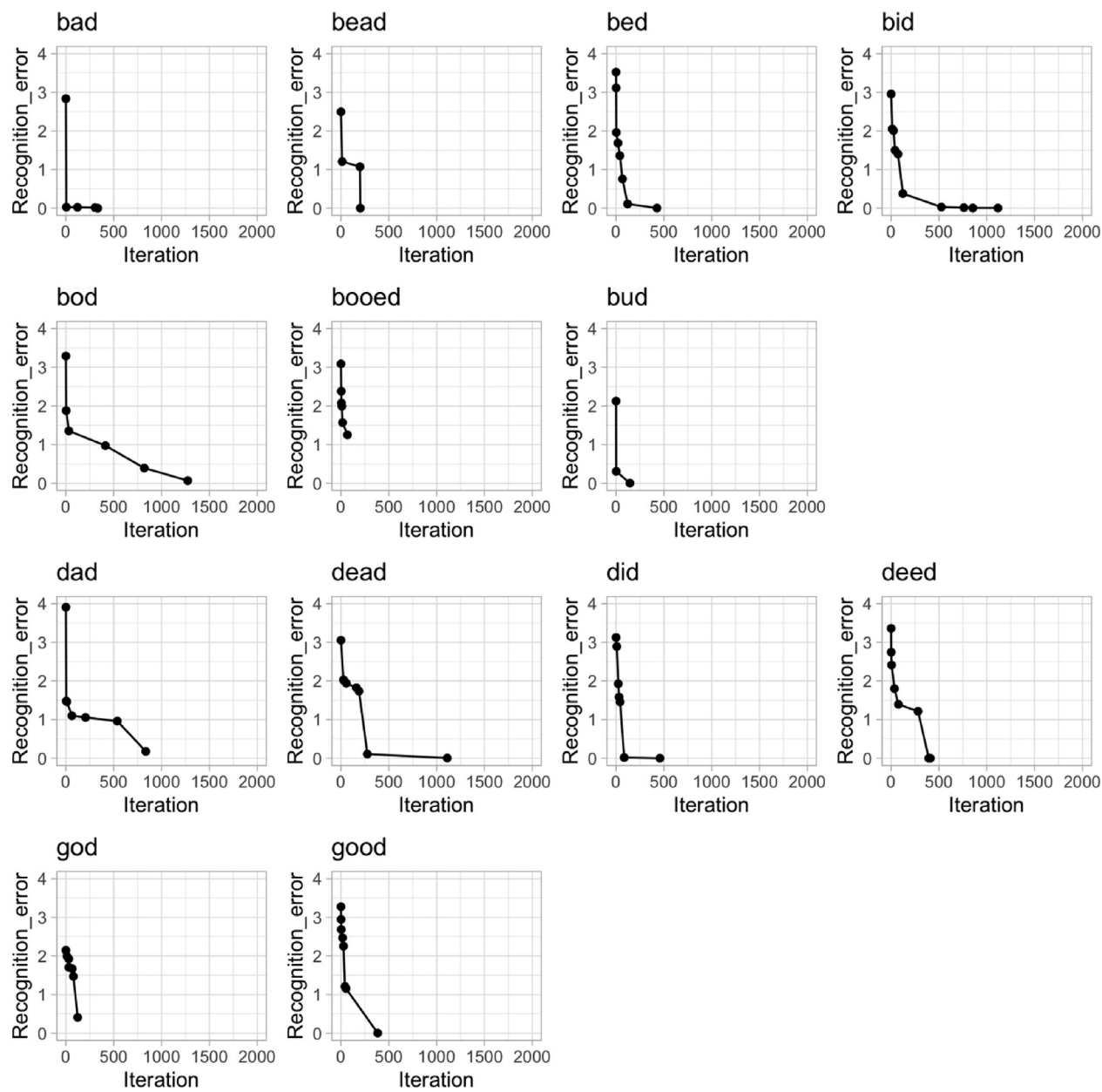
Fig. A5. Learning curves showing iterations with a lowering in the recognition error during the first stage of optimisation (random search).
