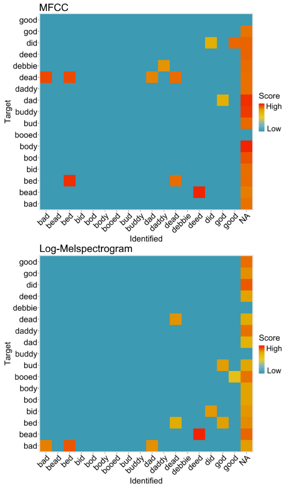
Fig. A1. Confusion matrices of words learned by adult vocal tract model when guided by MFCCs and Log Mel spectrograms, evaluated by a word recogniser. The score shows the weighted negative log likelihood loss. The two types of acoustic features resulted in very similar word error rates, that is, the intelligibility of the trained speech is indistinguishable.
