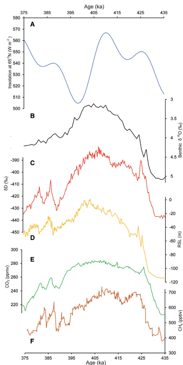
Fig. 1. The structure of MIS 11c as preserved in multiple palaeoclimatic records. A. Northern Hemisphere insolation (June 65°N) (Berger & Loutre 1991). B. LR04 stacked benthic \delta^{18}\text{O} record that broadly equates to global ice volume (Lisiecki & Raymo 2005). C. EPICA Dome C deuterium record of air temperature over Antarctica (Jouzel et al. 2007). D. Sea-level changes relative to present-day values (Rohling et al. 2010). E. High-resolution carbon dioxide record from EPICA Dome C (Nehrbass-Ahles et al. 2020). F. High-resolution methane record from EPICA Dome C (Nehrbass-Ahles et al. 2020).
