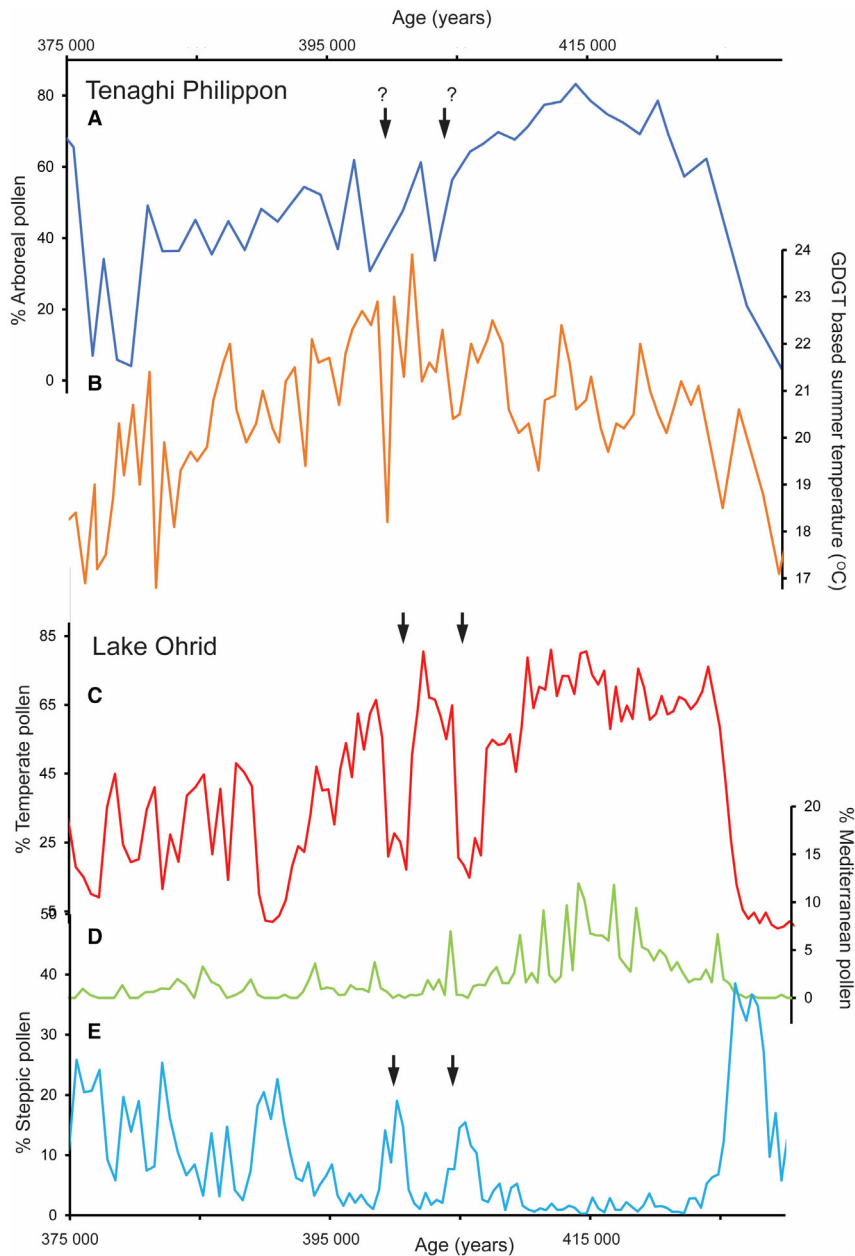
Fig. 7. Palaeoclimate records of MIS 11c from southeast Europe. A. Percentage arboreal pollen (minus Pinus , Betula and Juniperus ) from T. Philippon (Ardenghi et al. 2019). B. GDGT-based temperature reconstructions (Ardenghi et al. 2019). C–E. Percentage pollen data of different ecological groups from Lake Ohrid (Kousis et al. 2018).
