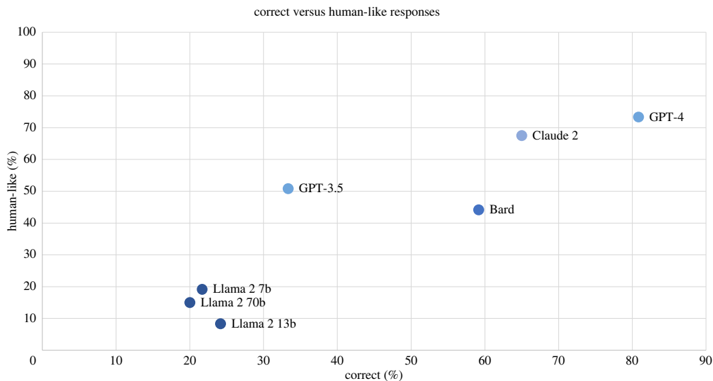
Figure 6. Proportion of correct versus human-like responses across all tasks for each language model. Correct responses include those with correct (logical) reasoning, as well as those with incorrect (illogical) reasoning that reached the correct answer. Human-like responses include those that are correct with logical reasoning, and those that are incorrect but are achieved through a studied human cognitive bias.
