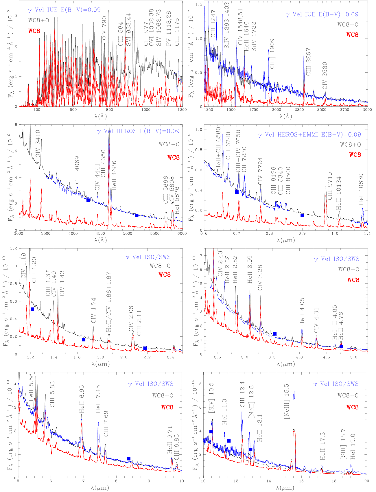
Figure 4. De-reddened UV IUE/HEROS spectroscopy (phase 0.5), calibrated optical ESO 50cm+HEROS and NTT+EMMI He I \lambda 10830 spectroscopy, ISO SWS infrared spectroscopy of \gamma Vel (blue), together with theoretical WC8+O model (black) and WC8 component (red), excluding correction for interstellar H I. Optical-IR photometry (Johnson et al. 1966; Williams et al. 1990; De Marco et al. 2000; Wright et al. 2010) is presented as blue boxes.
