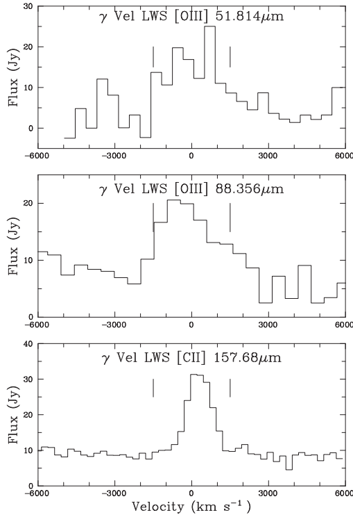
Figure 2. ISO -LWS spectrum of \gamma Vel, an average of back and forth scans, plotted in velocity space about a central wavelength [O III] 51.81 \mu\text{m} (top), [O III] 88.36 \mu\text{m} (centre), and [C II] 157.68 \mu\text{m} (bottom). Vertical lines indicate the expected extent of the stellar wind v_\infty = 1500 \text{ km s}^{-1} .
