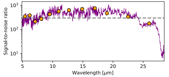
Figure 7. Measured S/N (rms) achieved with the JDISCS pipeline for the FZ Tau observation (purple curve). The dashed line indicates the expected goal of S/N = 300 . The orange circles show the prediction by the JWST ETC. Note that the division by the calibrator adds noise, which is included in the ETC prediction.
