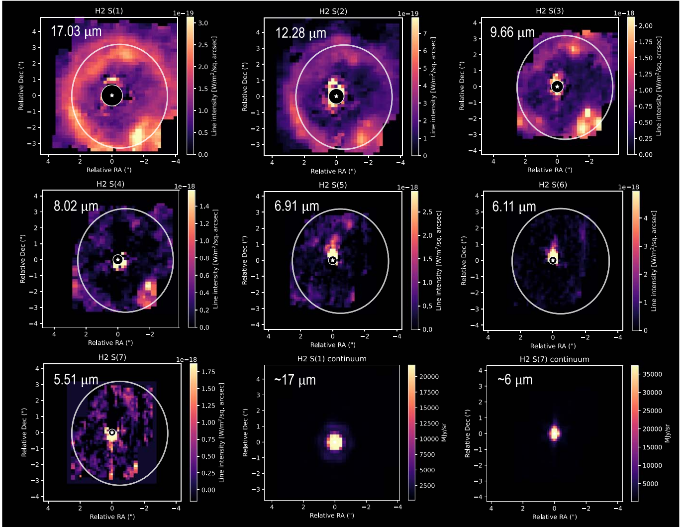
Figure 12. Continuum-subtracted line images of the rotational H 2 lines. The S(1) and S(2) images show the presence of a ring of cold H 2 emission, as well as a number of hot spots to the southwest of the star. The S(3) and S(4) lines are in Channel 2, which has a smaller FOV, and therefore these images do not include the full ring. Further, the Channel 1 FOV does not cover the hot spots. The inner working angle with radius of 1.22\lambda/D is masked, where D is the JWST telescope diameter and \lambda is the central wavelength of the line. The location of the star is indicated with a star symbol, and an ellipse is shown outlining the H 2 emission ring.
