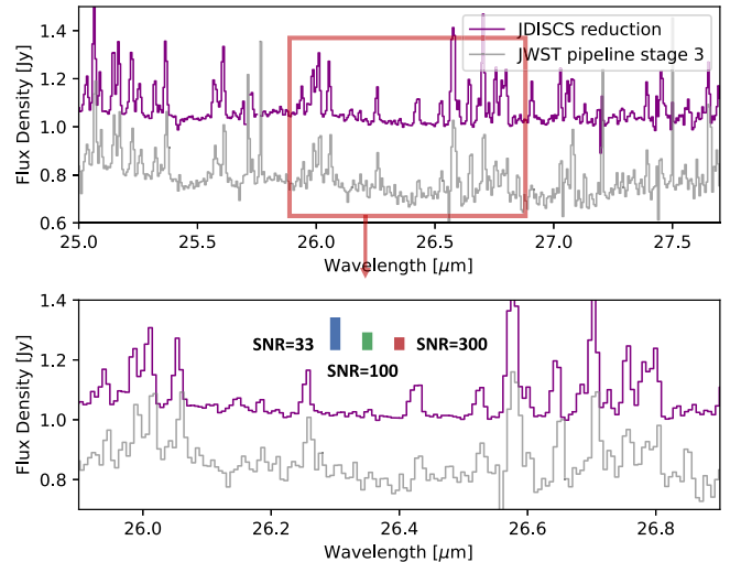
Figure 8. Comparison of the JDISCS reduction with the JWST pipeline for a section of Channel 4, which contains the lowest-energy water lines. Different levels of contrast ( S/N = 33, 100, \text{ and } 300 ) are indicated by bars showing \pm 1\sigma ranges. In the spectral range shown, the JDISCS spectrum reaches S/N \sim 300 , whereas the pipeline is limited by the calibration to S/N \sim 50 . The wavelength offsets in the JWST pipeline are apparent around 26 \mu\text{m} .
