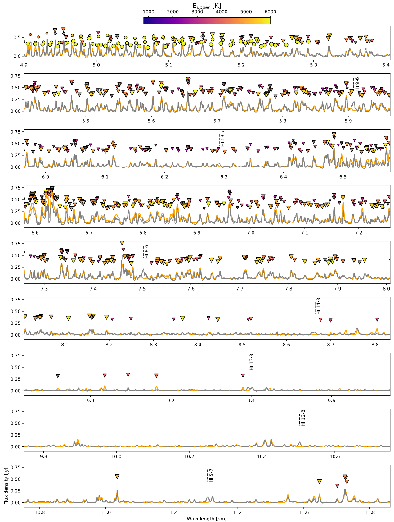
Figure 14. Continuum-subtracted emission-line spectrum of FZ Tau at \lambda < 11.85 \mu\text{m} . Bright \text{H}_2\text{O} lines are marked with triangles, CO lines with circles, and OH lines with stars. The colors and sizes of the symbols both show the upper-level energy of the transition in Kelvins. The orange curve shows the model fit to the spectrum (Table 4). The rovibrational lines are not used in the fit, but are displayed here at one-quarter of their predicted LTE flux from the model solution in Table 4, demonstrating a good match to the rotational populations, although the vibrational levels are subthermally populated. The remaining emission is dominated by H I recombination lines.
