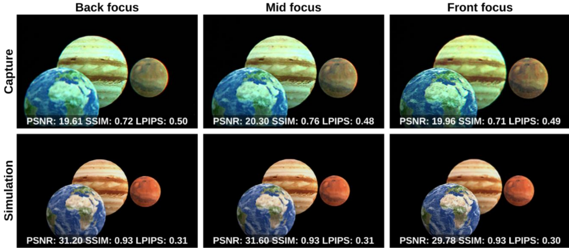
Figure 3. Experimental captures and simulation results of our method. There are six target image planes in depth with 1 mm separation between each depth plane (-2.5 mm and +2.5 mm with respect to an SLM).
