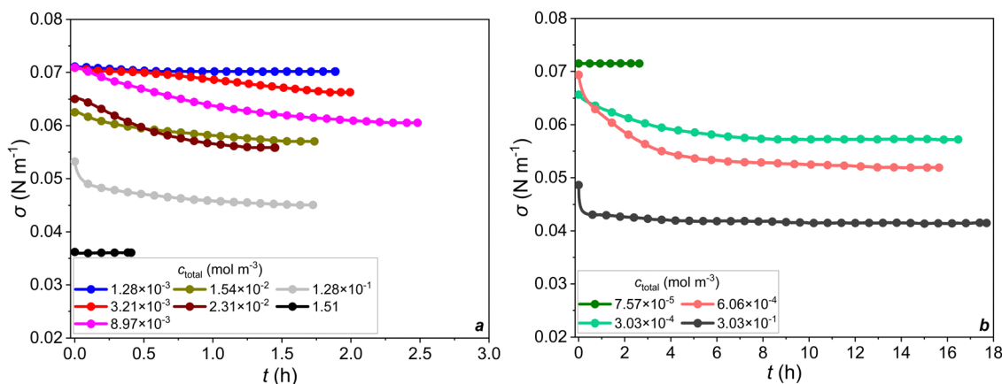
Fig. 4 Dynamic surface tension measurements for the (a) n_{\text{EOT}} = 0.01n_{\text{NaDDBS}} ( \text{CMC} = 1.06 \text{ mol m}^{-3} ), and (b) n_{\text{EOT}} = 4n_{\text{NaDDBS}} ( \text{CMC} = 9.10 \times 10^{-4} \text{ mol m}^{-3} ) premixed surfactant mixtures cases. The last curve in both graphs, represents total bulk concentrations above the CMC of the mixtures.
