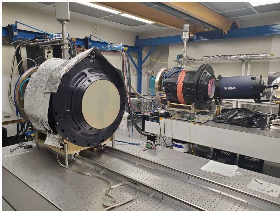
Figure 6. Two NIR cameras on the dual integration benches in the clean room at JHU. The first NIR Camera Unit (NCU SN1) with the fore-optics for the image quality investigation is shown on the far side (or on the right of this photo), while the second camera (NCU SN2) is in front of it (or on the left of this photo).
