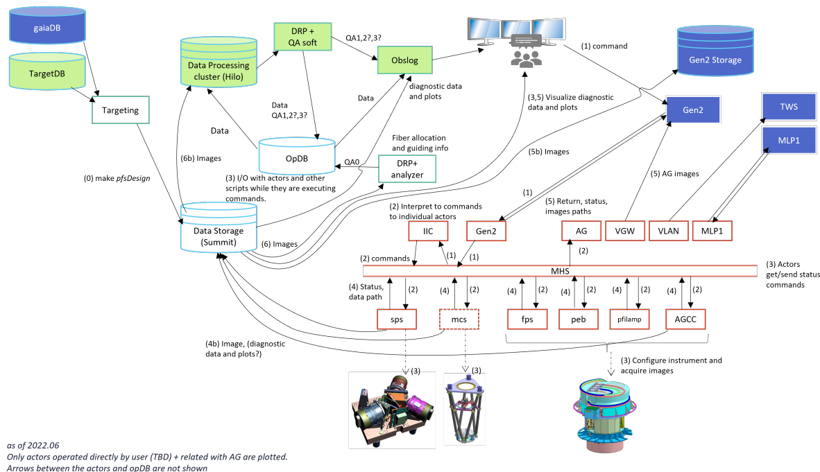
Figure 7. Schematic diagram of various software components and databases required for PFS operation.
