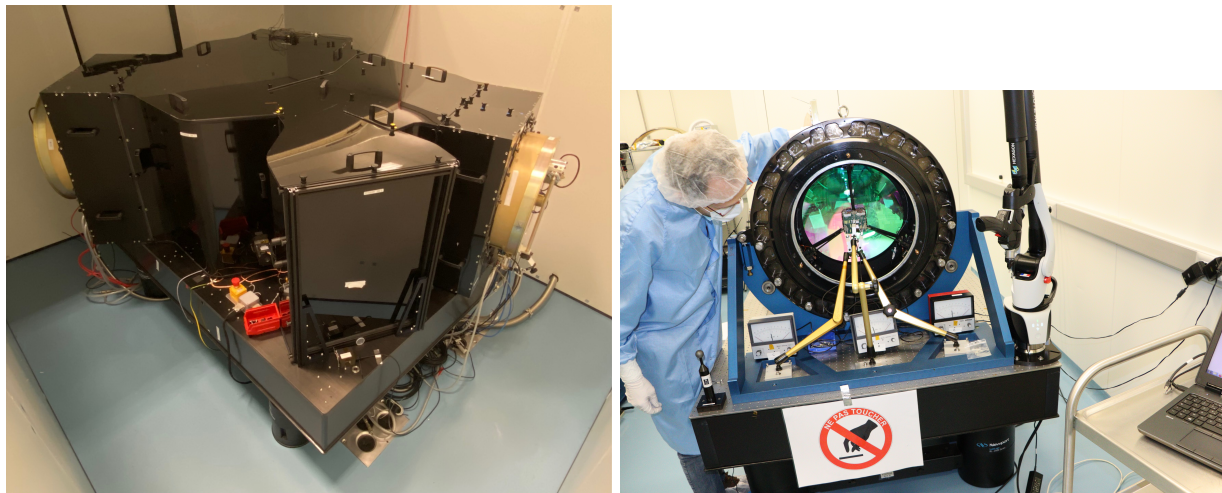
Figure 5. (Left) A spectrograph module assembled in the temperature controlled chamber. (Right) A metrology process for the visible camera focal plane geometry.
