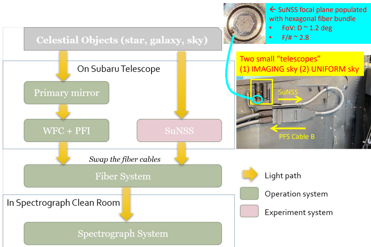
Figure 4. (Left) The block diagram of operation setup with PFI, and experimental setup with SuNSS. (Right) The actual hardware of SuNSS on the telescope spider together with Cable B1.
