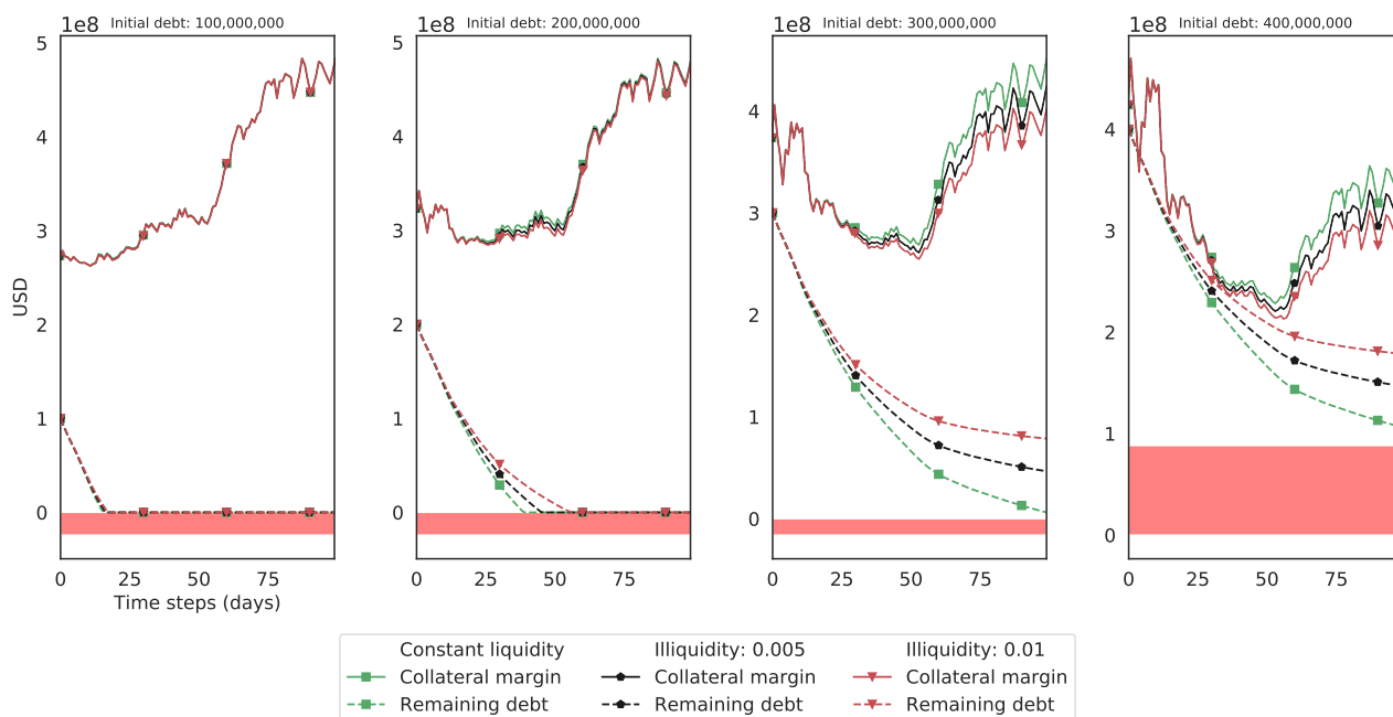
Figure 17: A DeFi lending protocol experiencing a sharp decline in the price of its collateral and reserve assets. Panels correspond to 4 different levels of system debt, with each panel showing the evolution of the collateral margin and the total debt outstanding. Each panel also shows the consequences of different liquidity parameters.
