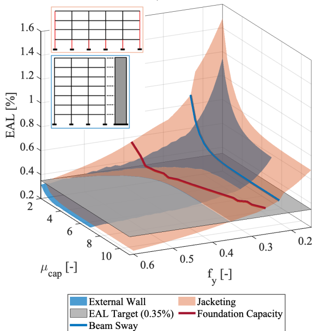
Figure 5: Direct loss-based retrofit used for conceptual design. Modified after Rubini et al. (2023)
