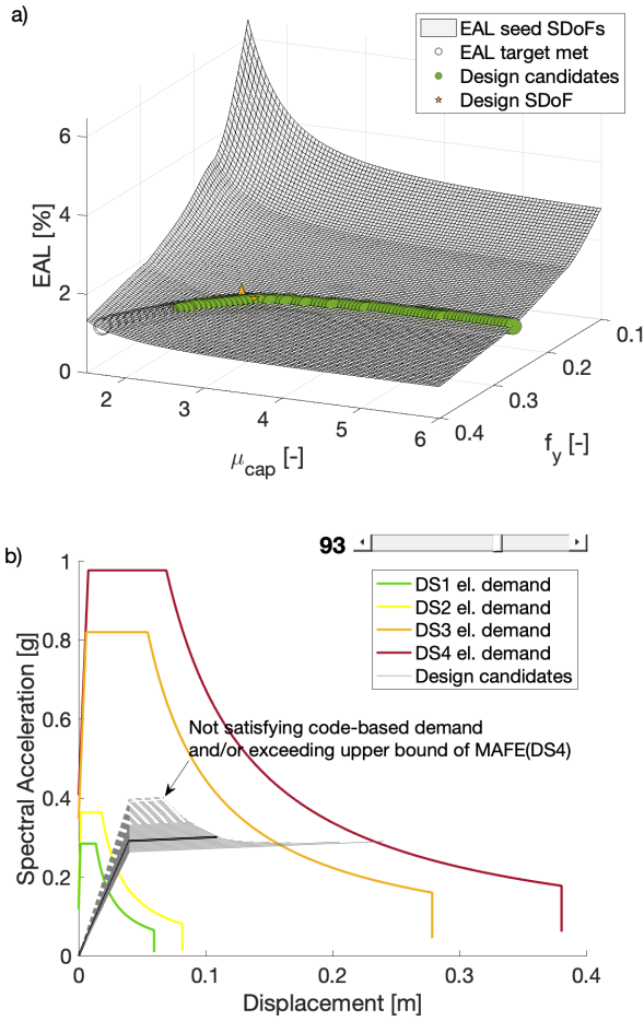
Figure 1: a) Expected annual loss of the seed SDoFs; b) capacity curves of the candidate design SDoFs. MAFE: mean annual frequency of exceedance; DS: damage state. Modified after Gentile and Calvi (2022)
