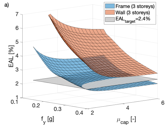
Figure 2: RC frame vs wall conceptual design for a 3-storey building using direct and indirect loss mapping (illustrative example). Modified after Gentile and Calvi (2022)
