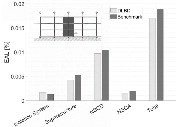
Figure 4: Direct loss-based design for a three-storey, RC medical clinic base-isolated with lead rubber bearings. Modified after Suarez et al. (2023)
