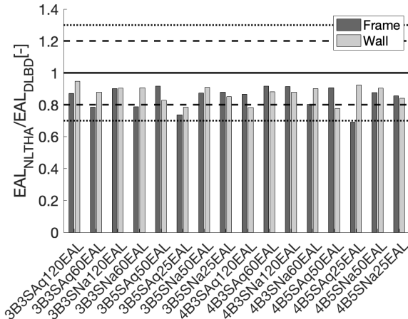
Figure 3: Ratio of NLTHA-based EAL versus the simplified DLBD-based one. Modified after Gentile and Calvi (2022)
