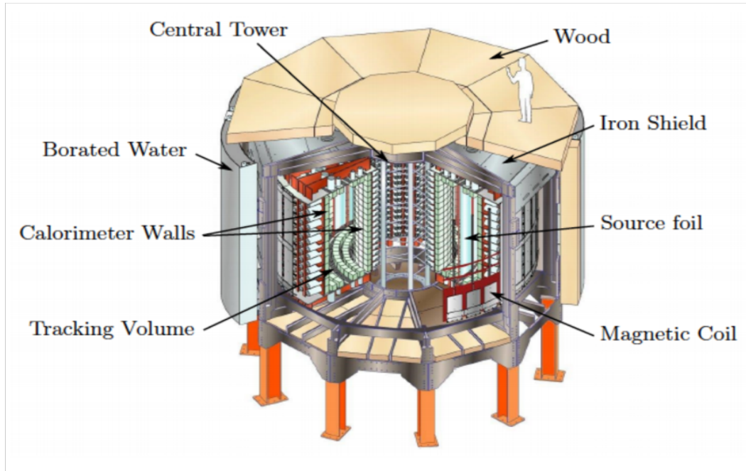
Figure 2.11: Open view of NEMO-3, illustrating the structure and the key components of the detector [61].
