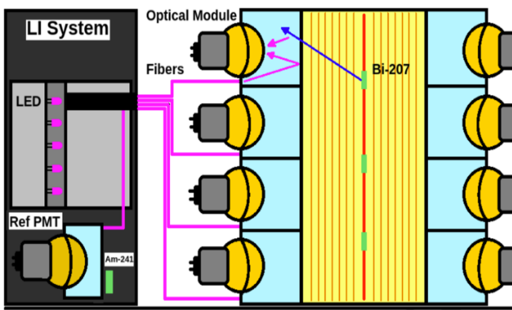
Figure 3.7: Illustration of the light injection monitoring system [121].
