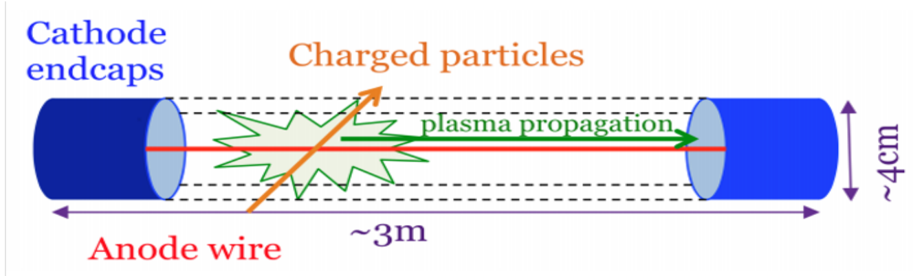
Figure 3.2: A SuperNEMO tracker cell illustrating detection principle [56].
