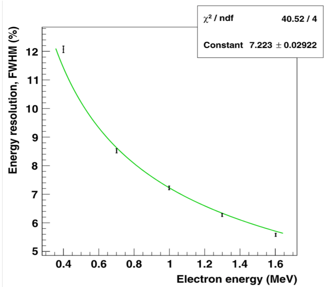
Figure 3.4: Energy resolution (FWHM %) as a function of the electron energy. Results were obtained using a ^{90}\text{Sr} based electron beam [60].
