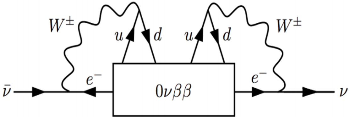
Figure 2.5: Feynman diagram for neutrinoless double beta decay ( 0\nu\beta\beta ), illustrating the Majorana nature of neutrinos for any intermediary decay mechanism [33].
