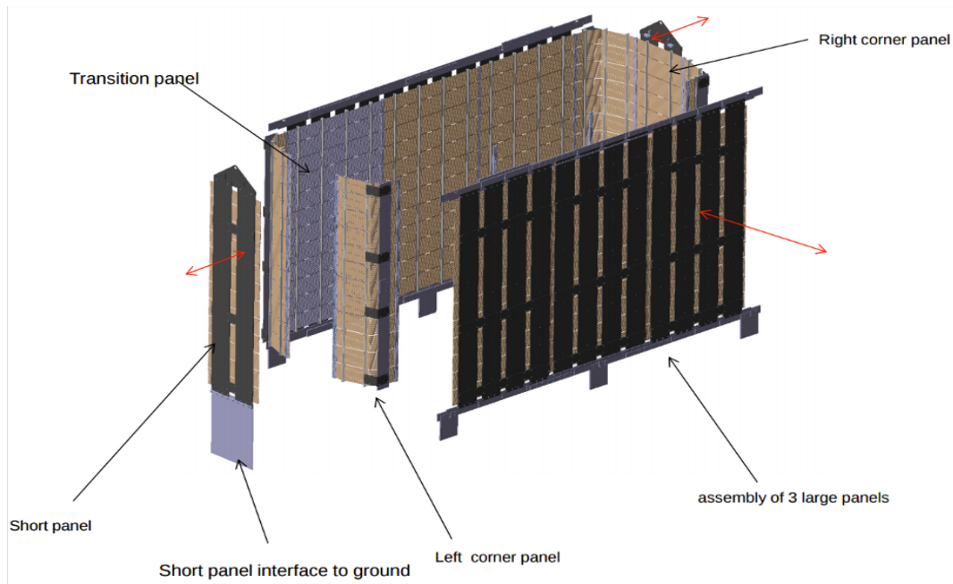
Figure 3.13: Open view of the magnetic coil illustrating the key components of the structure [122].
