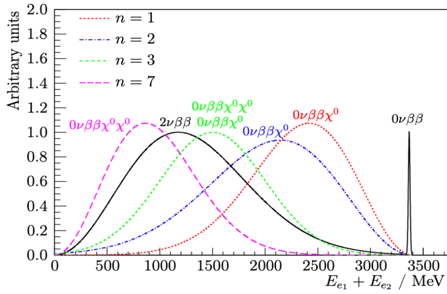
Figure 2.7: 0\nu\beta\beta and 2\nu\beta\beta energy spectra alongside four alternative Majoron decay modes with indices 1,2,3 and 7 [36]. Index n represents the different Majoron emitting modes that can be discerned from the shape of their energy spectra.
