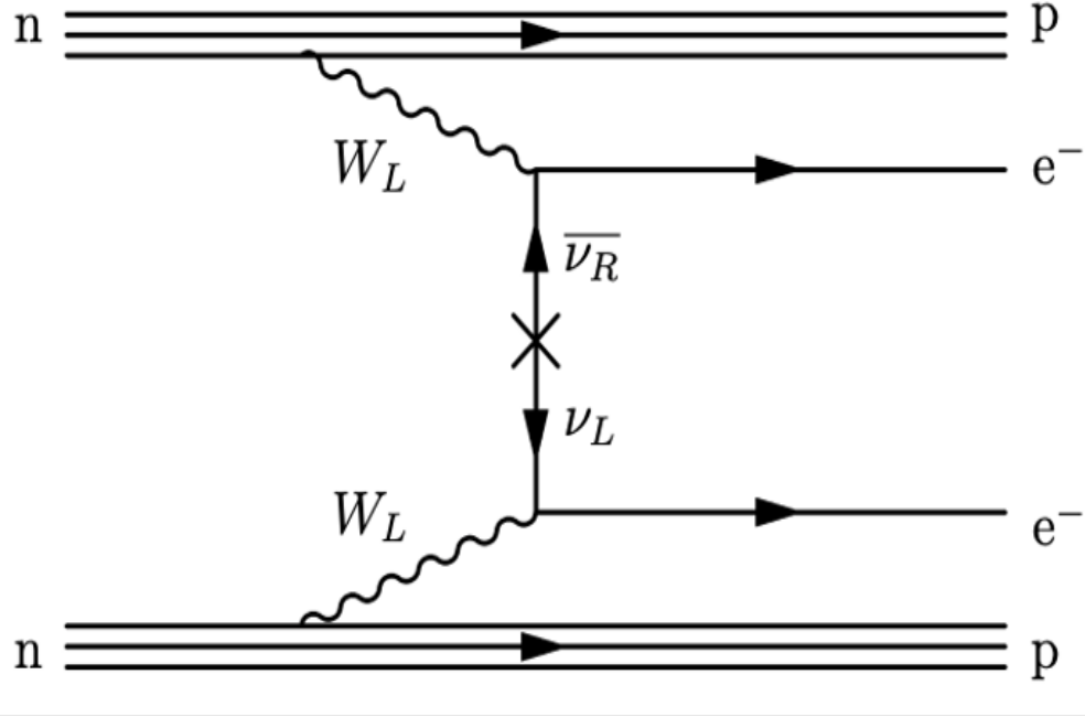
Figure 2.4: Feynman diagram for the forbidden neutrinoless double beta decay ( 0\nu\beta\beta ) via the light neutrino exchange (LNE) mechanism [8].
