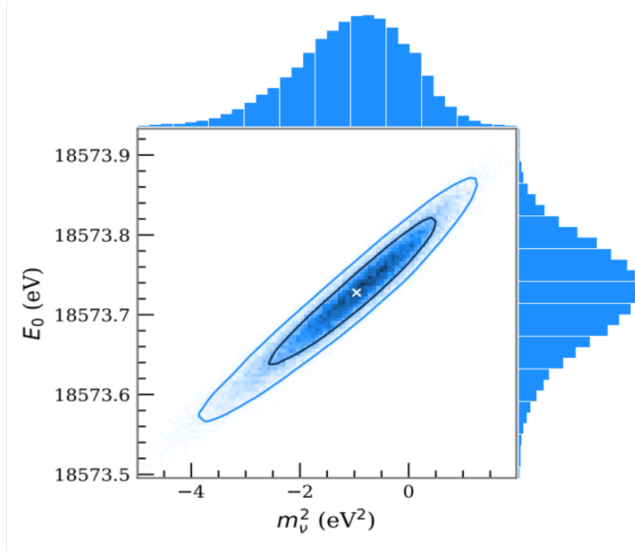
Figure 1.5: Scatter plot of the fit values for the neutrino mass squared and tritium \beta decay end point energy, including the 1- \sigma (black) and 2- \sigma (blue) error contours surrounding the best fit cross. The plot was developed using pseudo-experimental data [18].
