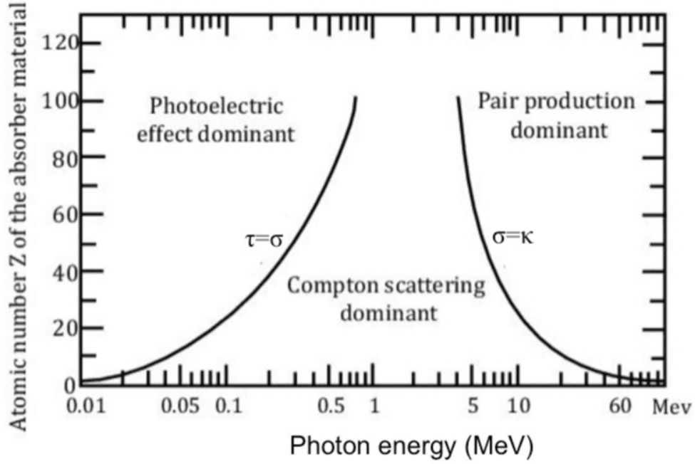
Figure 6.4: Cross section for photon interactions at various energies. The three principal interaction modes are shown as a function of the photon energy and atomic number of the interacting atom [52].
