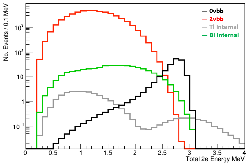
Figure 6.6: Energy spectra for 0\nu\beta\beta and the three internal backgrounds for events with a 2e topology under a uniform field. The internal backgrounds include 2\nu\beta\beta , ^{208}\text{Tl} and ^{214}\text{Bi} . The background spectra are normalised to exposure and the signal to the MDA half-life sensitivity.
