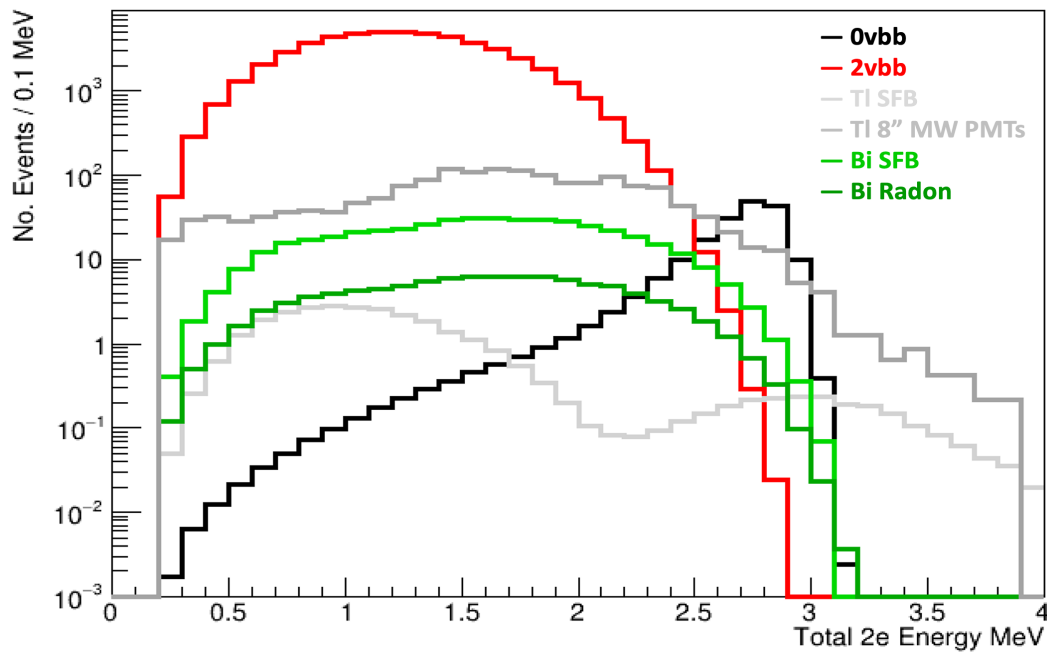
Figure 6.9: Energy spectra for 0\nu\beta\beta , 2\nu\beta\beta , ^{208}\text{Tl}/^{214}\text{Bi} in the source foil bulk (SFB), ^{208}\text{Tl} on the 8'' Main Wall PMT glass bulb (8'' MW PMTs), ^{214}\text{Bi} from the combined radon sources for events with a 2e topology and no magnetic field. The background spectra are normalised to the exposure and the signal to the MDA half-life sensitivity.
