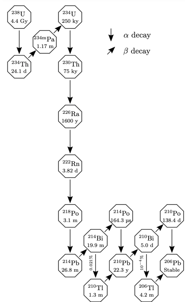
Figure 3.10: ^{238}\text{U} decay chain, known as the radium series. The same notation is used between this Figure and Figure 3.9 [8].
