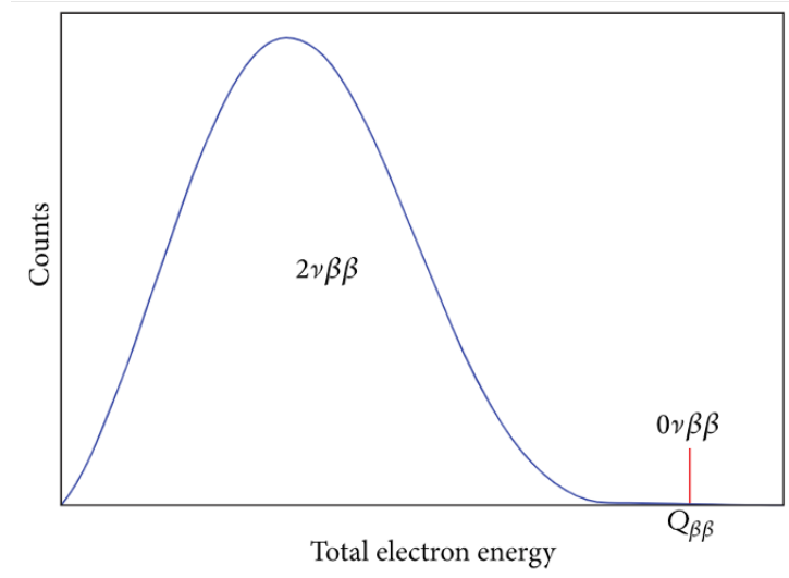
Figure 2.3: 0\nu\beta\beta and 2\nu\beta\beta theoretical electron energy spectra. 0\nu\beta\beta is represented by a single monochromatic line [32].
