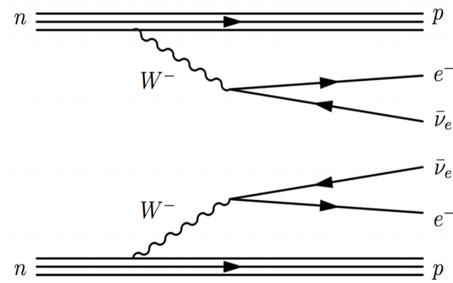
Figure 2.2: Feynman diagram for the Standard Model two neutrino double beta decay ( 2\nu\beta\beta ) [8].
