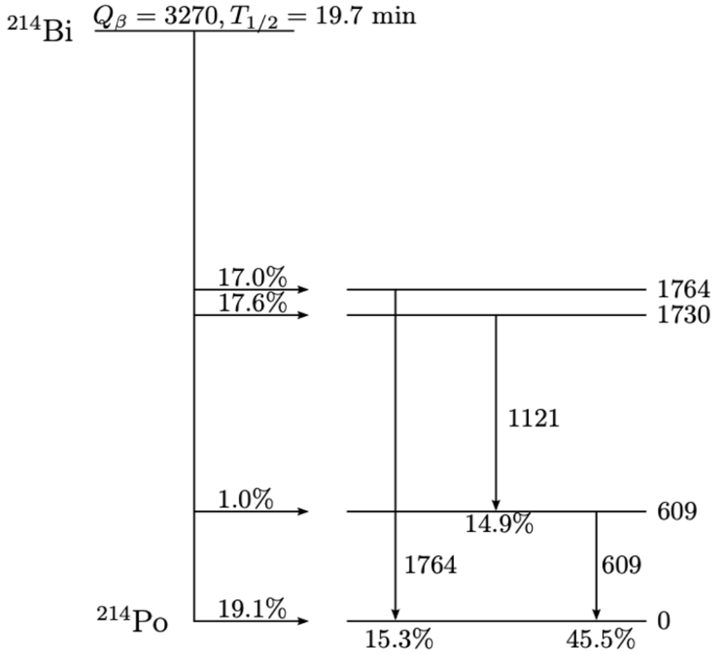
Figure 6.2: Simplified decay scheme for ^{214}\text{Bi} undergoing beta decay into ^{214}\text{Po} , illustrating the most common transition lines, with the energies in keV [8].
