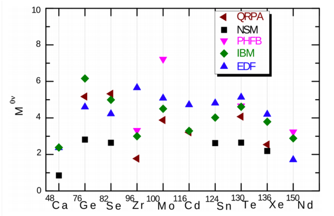
Figure 2.10: Nuclear matrix element (NME) values for the main double beta decaying isotopes used for experimentation, using the different methods described in Section 2.4 [45].
