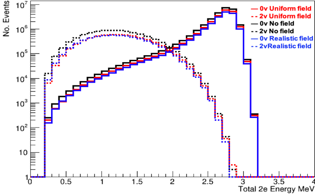
Figure 5.1: 0\nu\beta\beta and 2\nu\beta\beta total energy spectra for events with a 2e topology with all three magnetic fields. The 0\nu\beta\beta spectra are illustrated by the thick line and 2\nu\beta\beta by the dotted line. The spectra are normalised to the number of simulated events.
