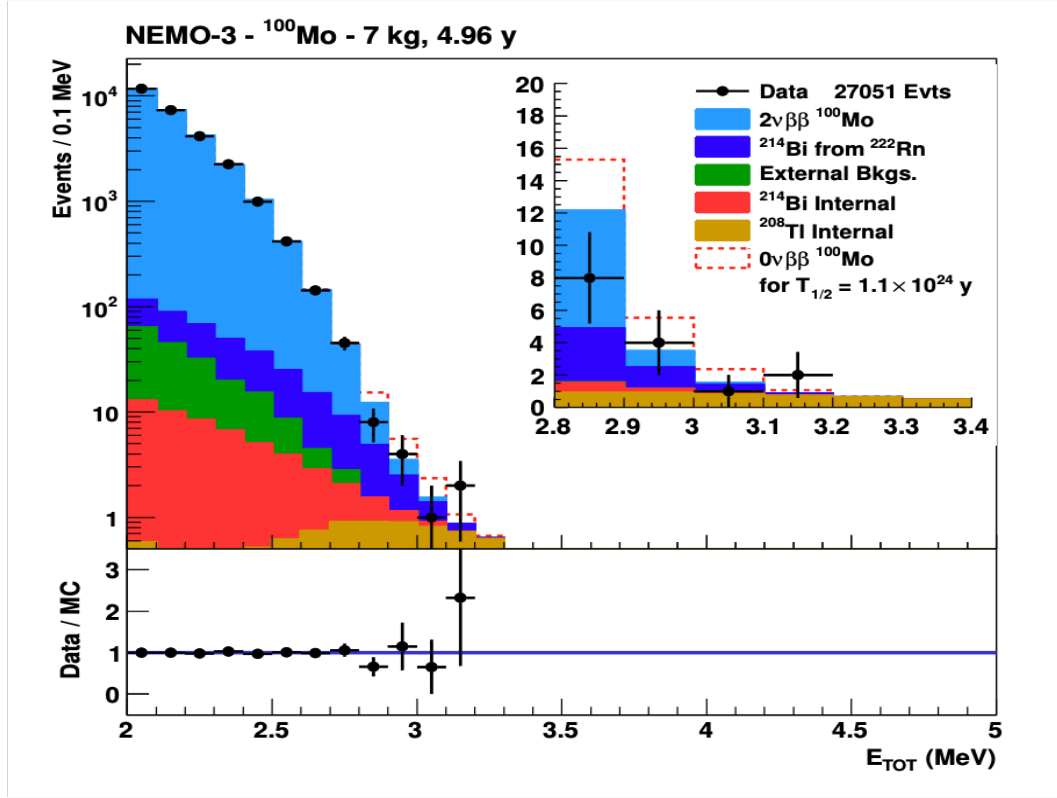
Figure 2.14: Energy distribution of ^{100}\text{Mo} double beta candidate events as well as the background contributions in the ^{100}\text{Mo} ROI [107]. The exposure for ^{100}\text{Mo} is 34.4 kg yrs.
