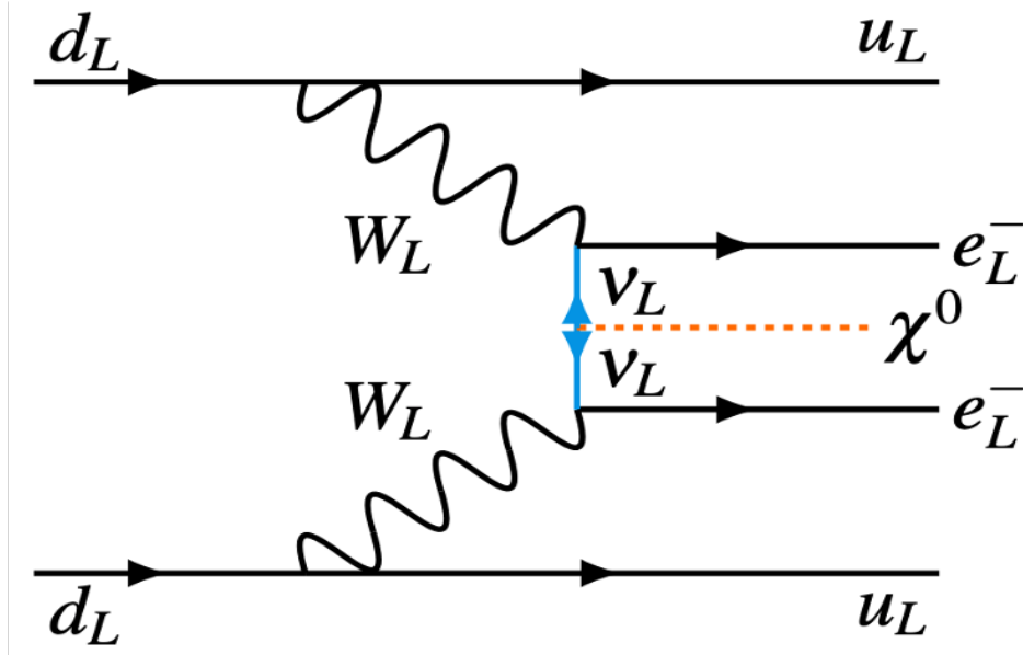
Figure 2.6: Feynman diagram for the forbidden neutrinoless double beta decay ( 0\nu\beta\beta ) via the emission of an associated Majoron ( \chi^0 ) [35].
