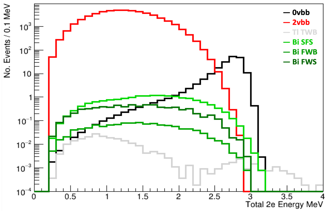
Figure 6.7: Energy spectra for 0\nu\beta\beta , 2\nu\beta\beta , the two radon backgrounds and ^{208}\text{Tl}/^{214}\text{Bi} in the tracker wire bulk (TWB), for events with a 2e topology under a uniform field. The radon backgrounds include ^{214}\text{Bi} on the source foil surface (SFS) and field wire bulk/surface (FWB/FWS). The background spectra are normalised to the exposure and the signal to the MDA half-life sensitivity.
