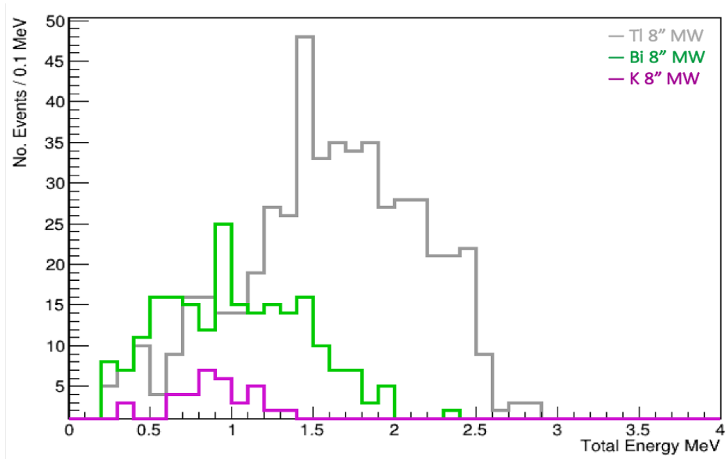
Figure 6.8: Energy spectra for all 8" Main Wall (MW) backgrounds with a 2e topology and no magnetic field, including ^{208}\text{Tl} , ^{214}\text{Bi} and ^{40}\text{K} . For ^{214}\text{Bi} and ^{40}\text{K} , no events with a 2e topology were found in the ^{82}\text{Se} ROI. The energy spectra is normalised to the total number of simulated events.
