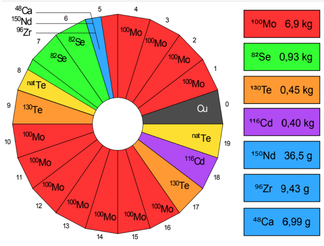
Figure 2.13: Distribution of source material across the 20 sections of the NEMO-3 detector [107].
