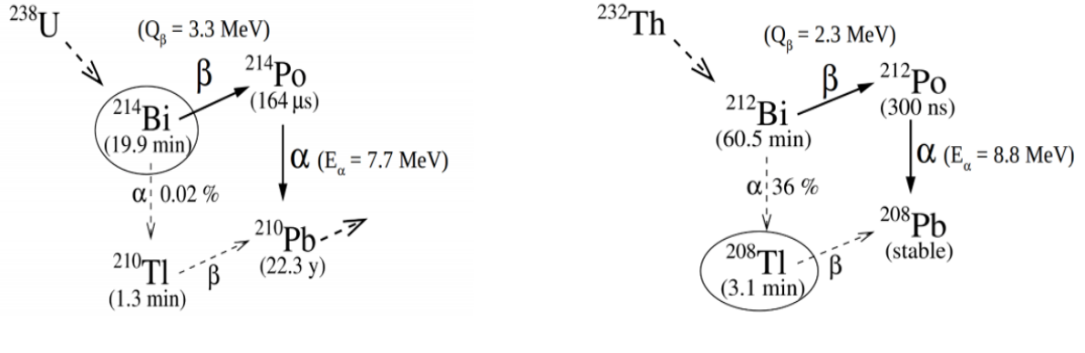
Figure 3.11: The two cascades, ^{214}\text{Bi} \rightarrow ^{214}\text{Po} and ^{212}\text{Bi} \rightarrow ^{212}\text{Po} , used to determine the contamination of ^{214}\text{Bi} and ^{208}\text{Tl} respectively [118].
