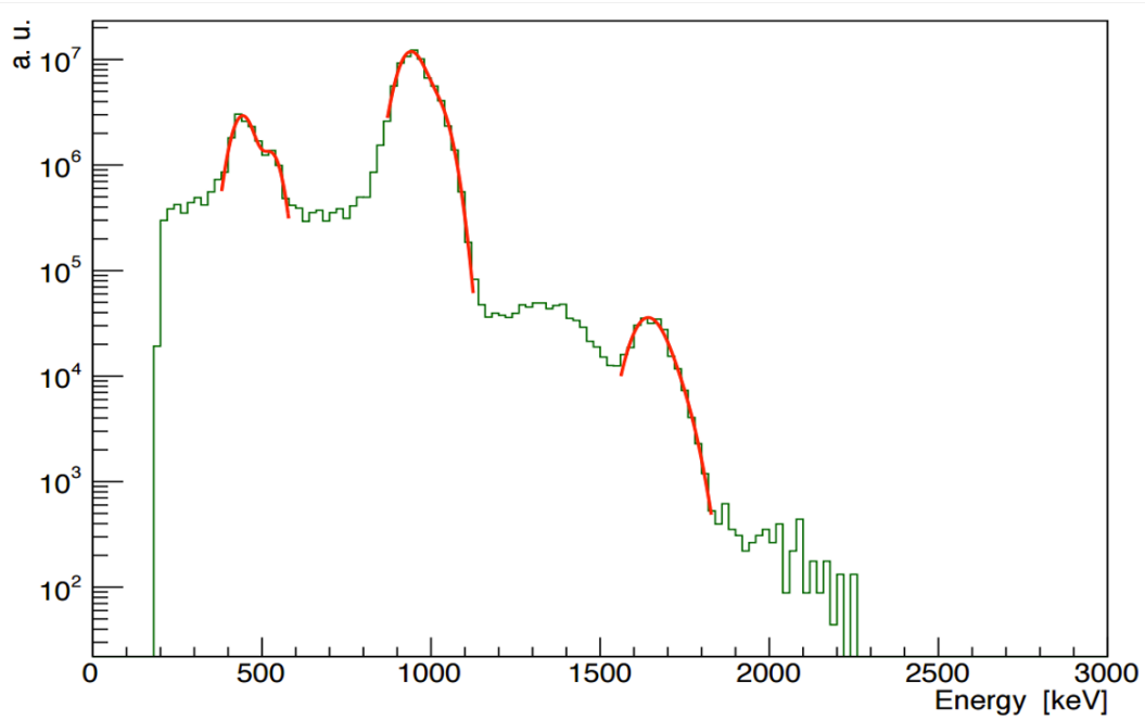
Figure 3.6: Reconstructed ^{207}\text{Bi} energy spectrum from a simulated calibration run. The three peaks correspond to the 482, 976 and 1682 keV energy lines [120] (shown with arbitrary units a.u. on the y axis).
