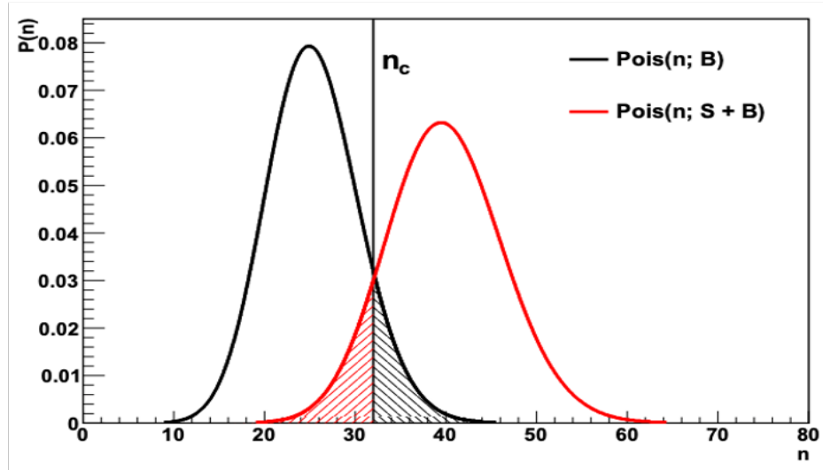
Figure 4.10: Probability distributions for the two Poisson variables, B and S+B . The black curve represents the background distribution and the red curve signal + background, with the shaded areas each corresponding to 1 - \text{CL} [8].
