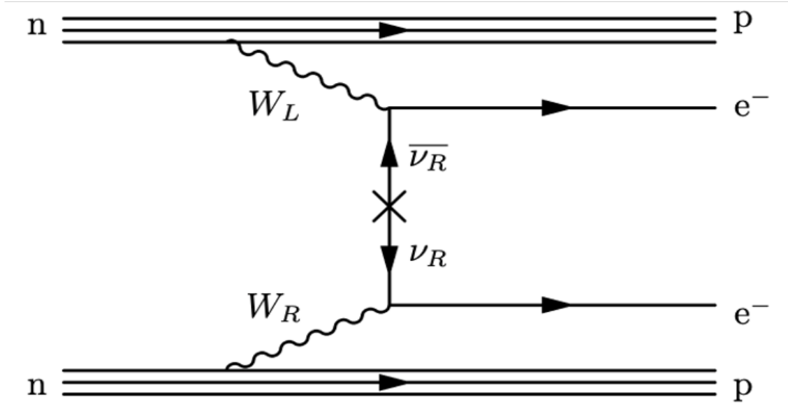
Figure 2.8: Feynman diagram for the forbidden neutrinoless double beta decay ( 0\nu\beta\beta ) via the \langle\lambda\rangle right handed weak current mechanism [34].
