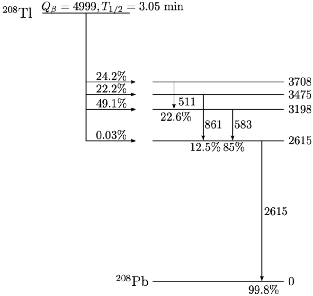
Figure 6.1: Simplified decay scheme for ^{208}\text{Tl} undergoing beta decay into ^{208}\text{Pb} , illustrating the most common transition lines, with the energies in keV [8].
