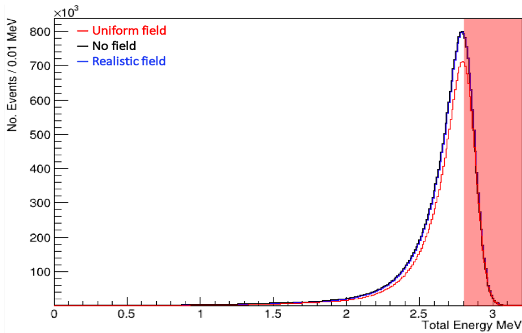
Figure 4.9: 0\nu\beta\beta total energy spectra for the three magnetic field configurations, with the region of interest (2.8 - 3.2 MeV) highlighted in red. The theoretical ROI is above the peak due to energy losses in the detector.
