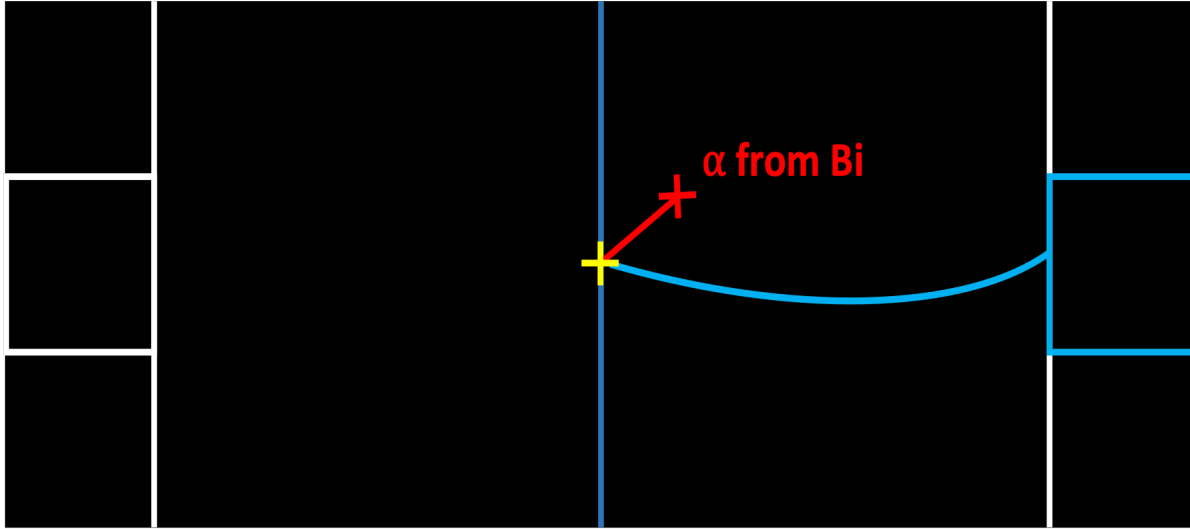
Figure 4.7: Representation of a reconstructed event with one electron (blue track) as well as an alpha (short red track), from a ^{214}\text{Bi} or ^{212}\text{Bi} alpha decay, with an initial decay vertex on the source foil.
