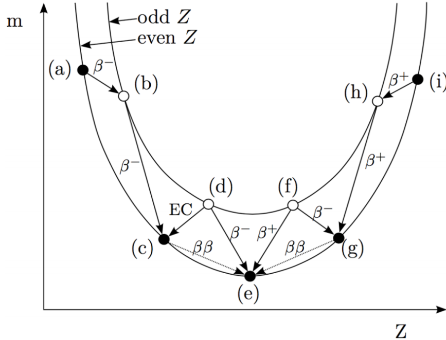
Figure 2.1: SEMF predictions for even values of A . The permitted decays are represented by arrows, with the decay mode labelled for each transition [8].
