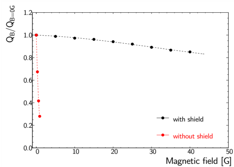
Figure 3.14: Photoelectron collection efficiency as a function of magnetic field strength. Data was collected using SuperNEMO PMTs [123].
