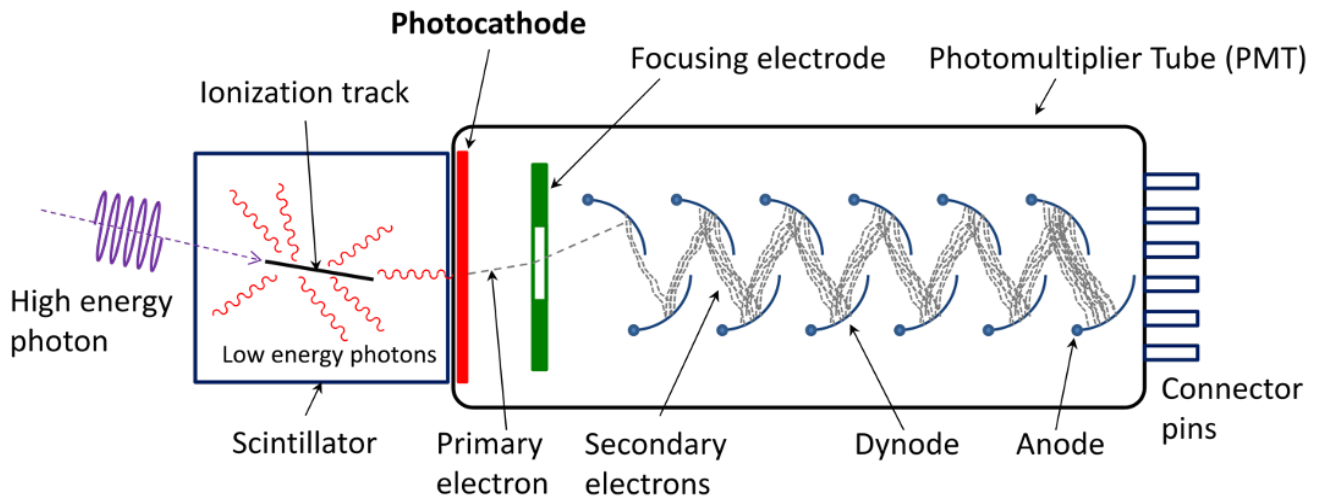
Figure 3.15: Schematic view of the working principle of a PMT coupled to a scintillator. The scintillation photons are focused within the PMT and read as an electric signal at the anode [124].
