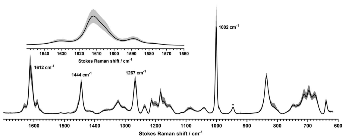
Fig. 1 Raman data ( \lambda = 785 nm line laser, 20\times NA = 0.40 objective) collected on the ETFE- g -poly(VBC) intermediate membrane (DoG = 73%) used to produce the MPIP(LEX) and MPIP(1.1) in this study. This data is derived from n = 100 individual spectra recorded at random locations across both surfaces of the membrane. The black line represents the averaged (mean) spectra. The grey envelope shows the range of intensities recorded at each Raman shift (minimum to maximum values obtained). *Spectral intensities were normalised to the ETFE-derived band at 945 \text{cm}^{-1} to aid visual comparison. The inset presents more detail around the 1612 \text{cm}^{-1} band from the poly(VBC) grafted chains. Cosmic rays were not removed (see grey peak at 920 \text{cm}^{-1} ).
